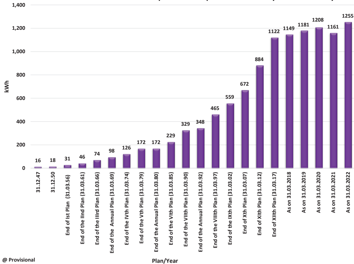
Chart : 4 Planwise Growth of Per Capita Consumption of Electricity in the Country
