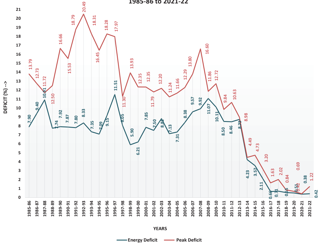
All India Peak and Energy Deficit (Utilities) 1985-86 to 2021-22
