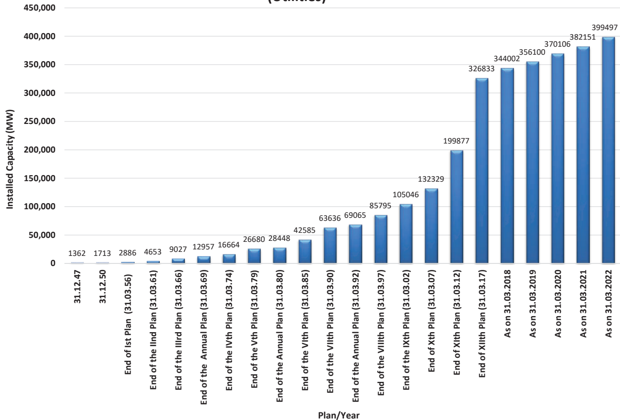
Planwise Growth of Installed Capacity in the Country (Utilities)
