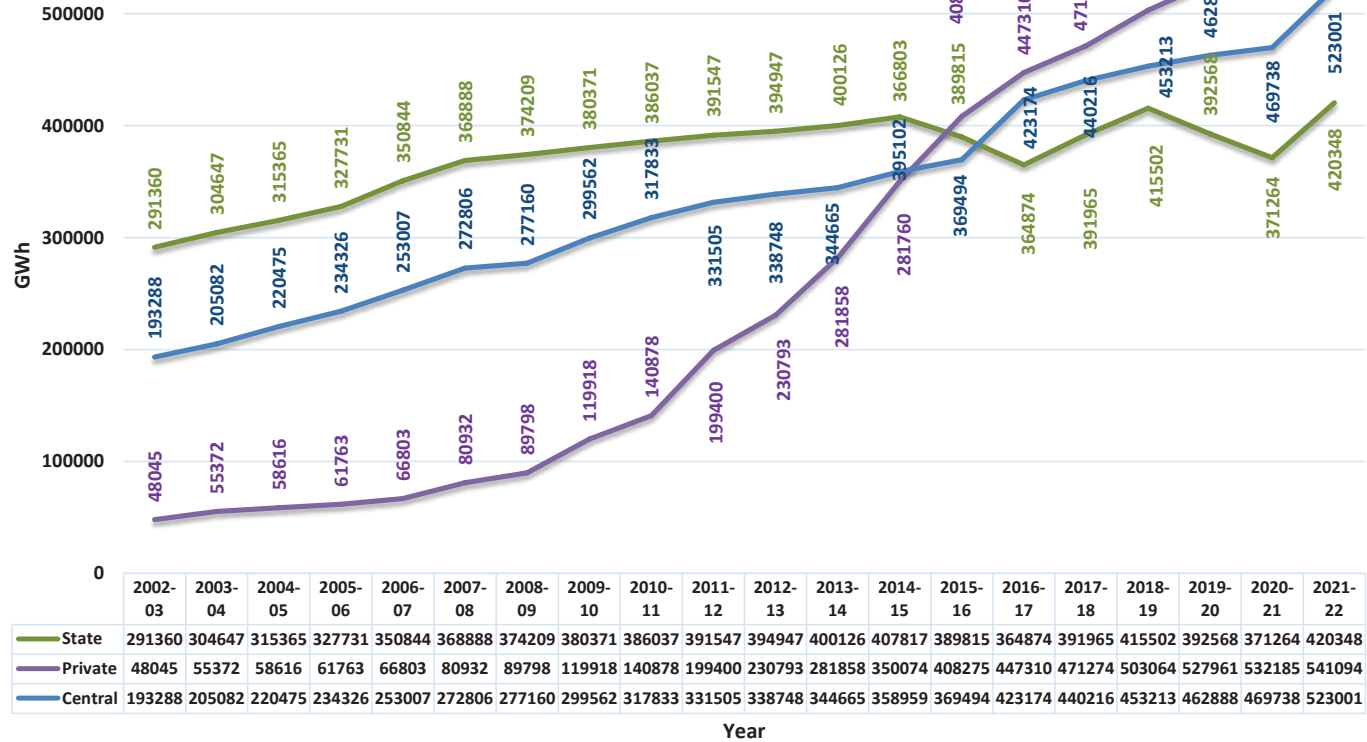
Sector wise Growth of Energy Generation (GWh) 2002-03 to 2021-22
