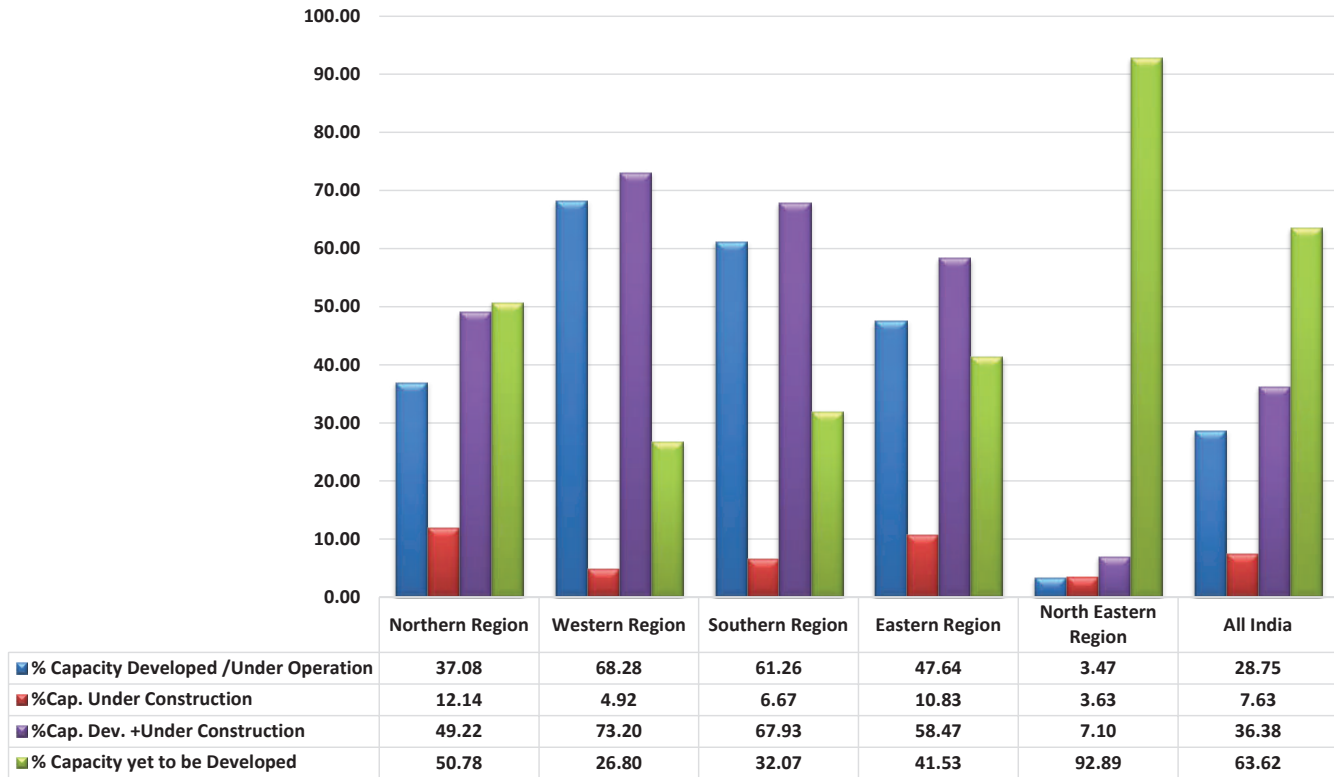
Regionwise Status of Hydro Electric Potential Development Chart : 6B In terms of Installed Capacity above 25 MW % wise (As on 31.03.2022 )
