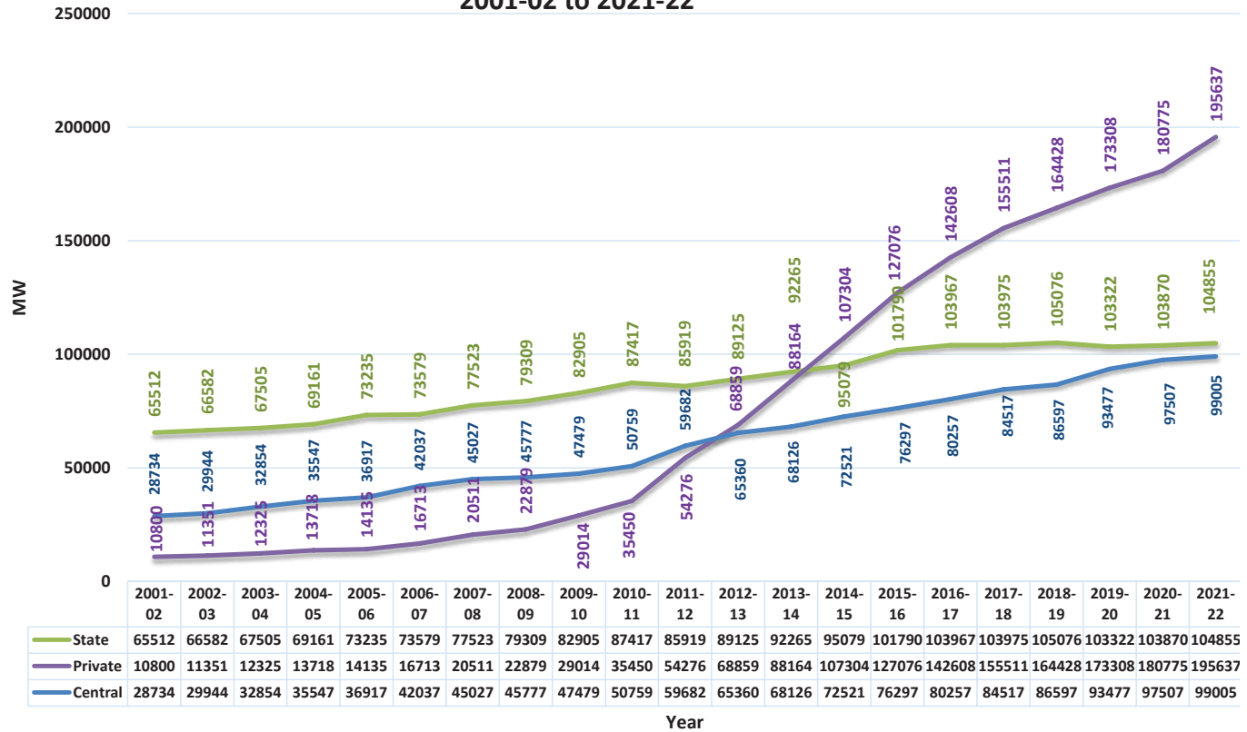
Sector wise Growth of Installed Capacity (MW) 2001-02 to 2021-22
