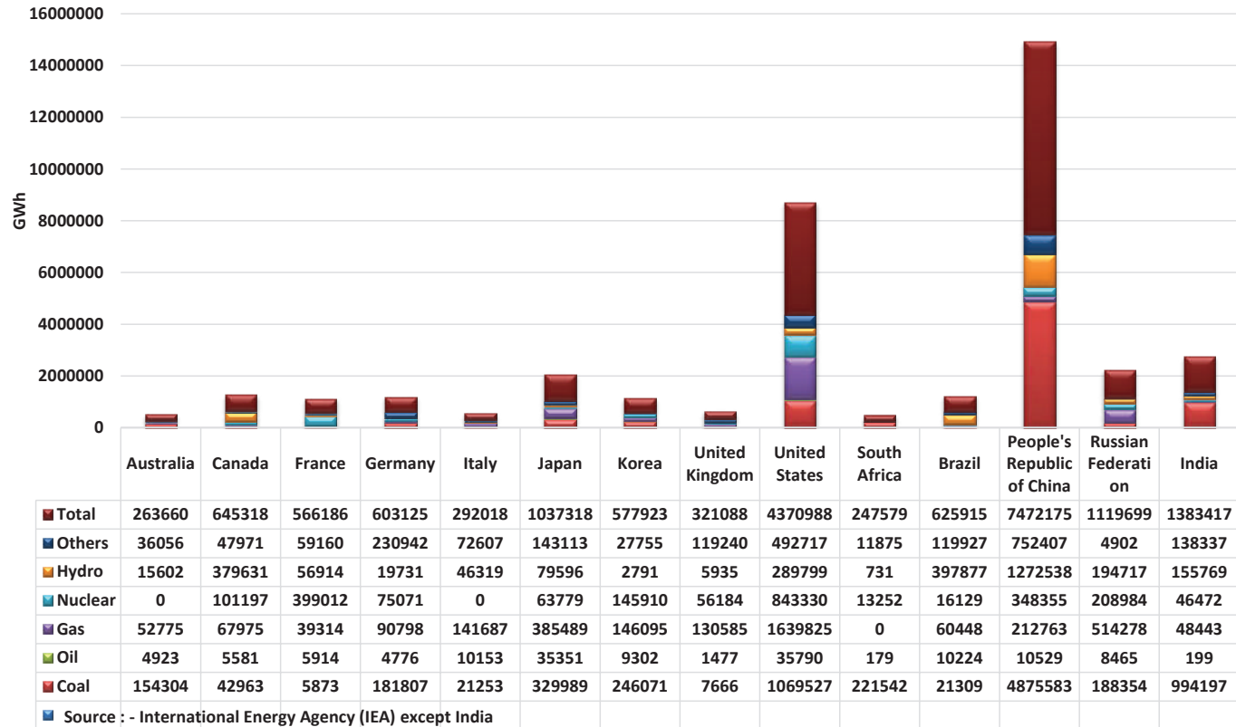
Gross Electricity Generation in various Countries Mode- Wise in 2019
