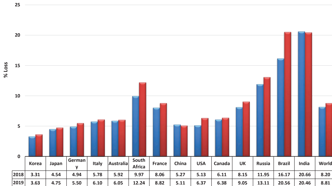
T & D Losses of Various Countries in 2018 & 2019 (%)
