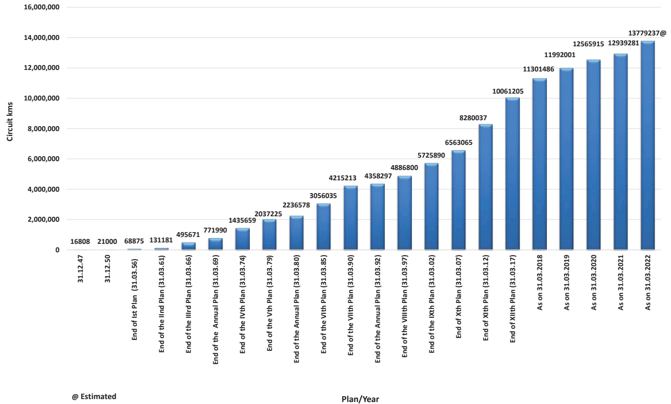
Planwise Growth of Transmission Lines in the Country below 66 kV
