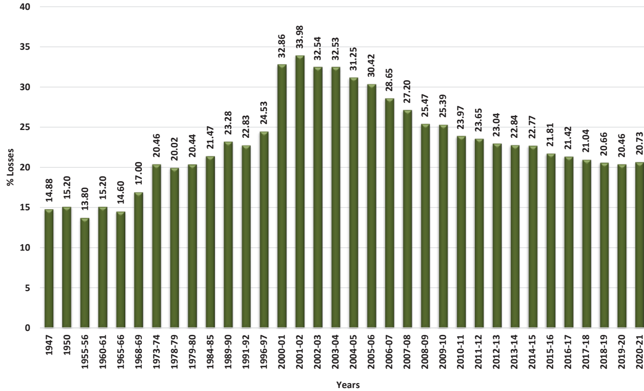
All India Transmission and Distribution Losses (%)
