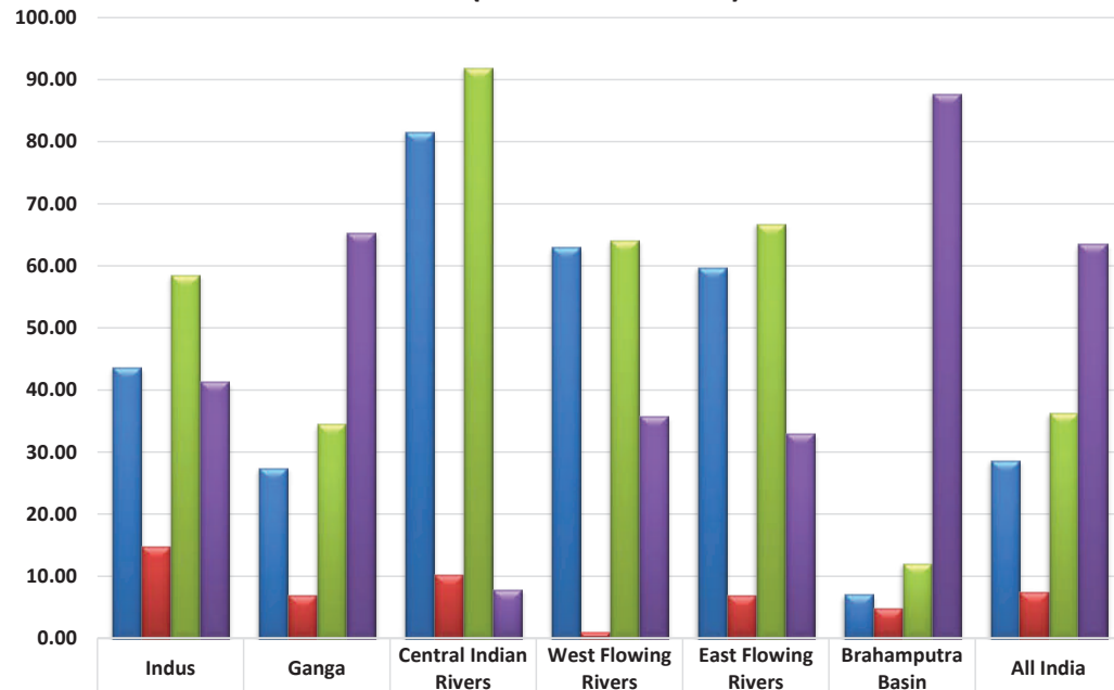
Basinwise Status of Hydro Electric Potential Development Chart : 6A In terms of Installed Capacity above 25 MW % wise (As on 31.03.2022)
