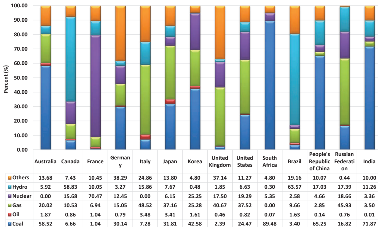
Mode wise % Share in Electricity Generation in various Countries in 2019
