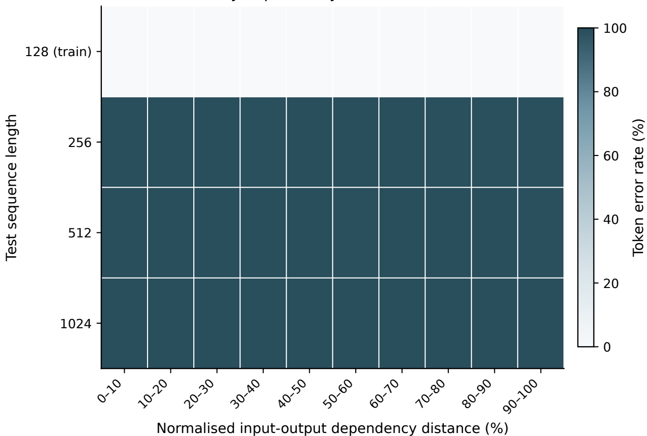
Reverse: error by dependency distance (Learned, seed 42)
