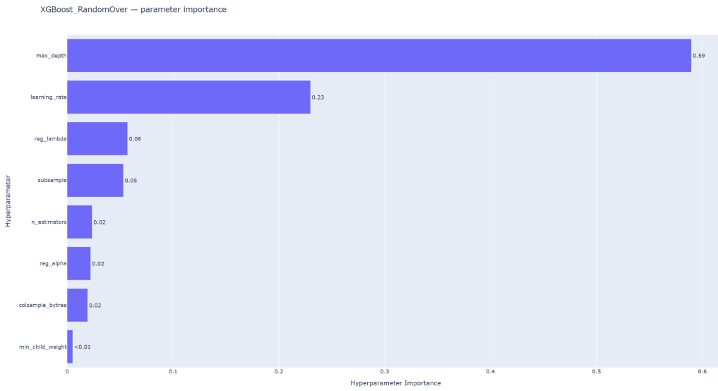
Figure 8: Optuna parameter importance plot of XGBoost + RandomOver (0.5188)
