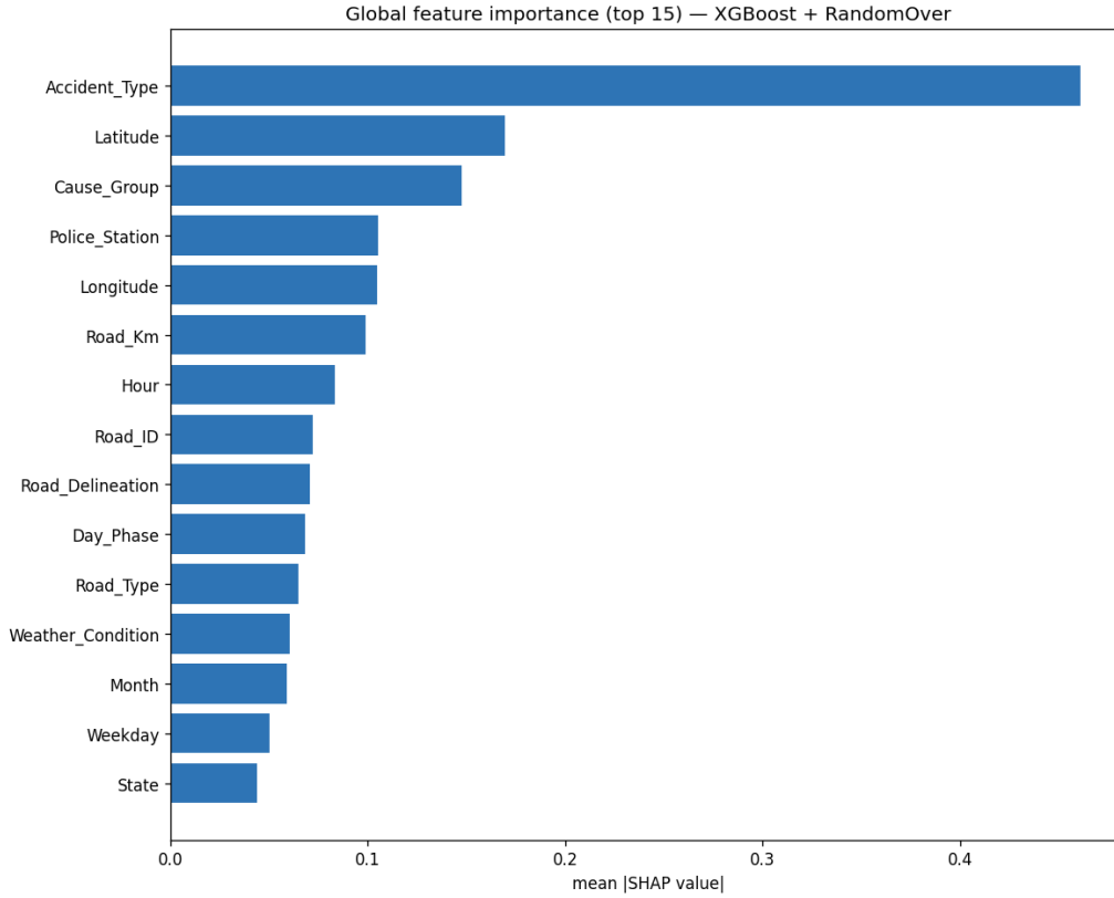
Figure 9: Top 15 features ranked by mean absolute SHAP value, displayed in a bar chart
