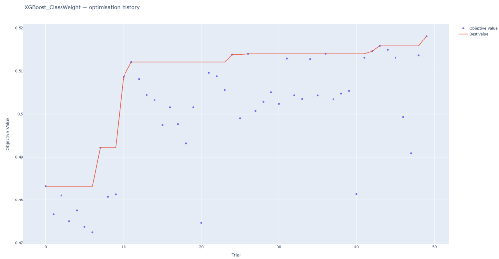
Figure 13: XGBoost ClassWeight history plot
