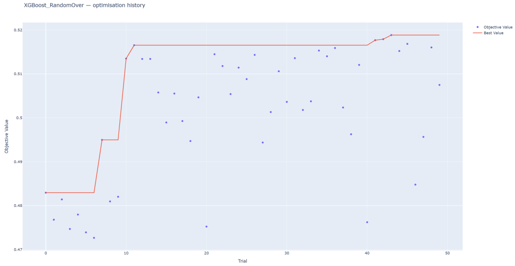
Figure 7: Optuna optimisation history plot of XGBoost + RandomOver (0.5188)
