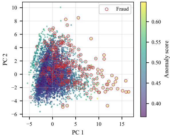
(b) Test sample, PCA projection
