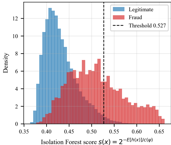
(a) Score distribution
