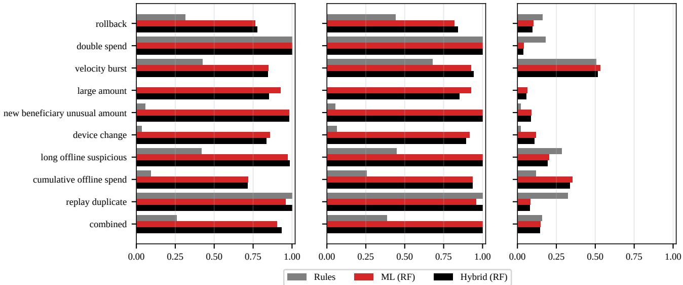
(a) Recall (transactions)
