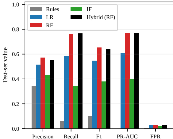
(a) Repo-native features/rules
