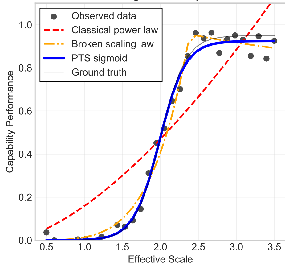
A. Scaling Law Comparison
