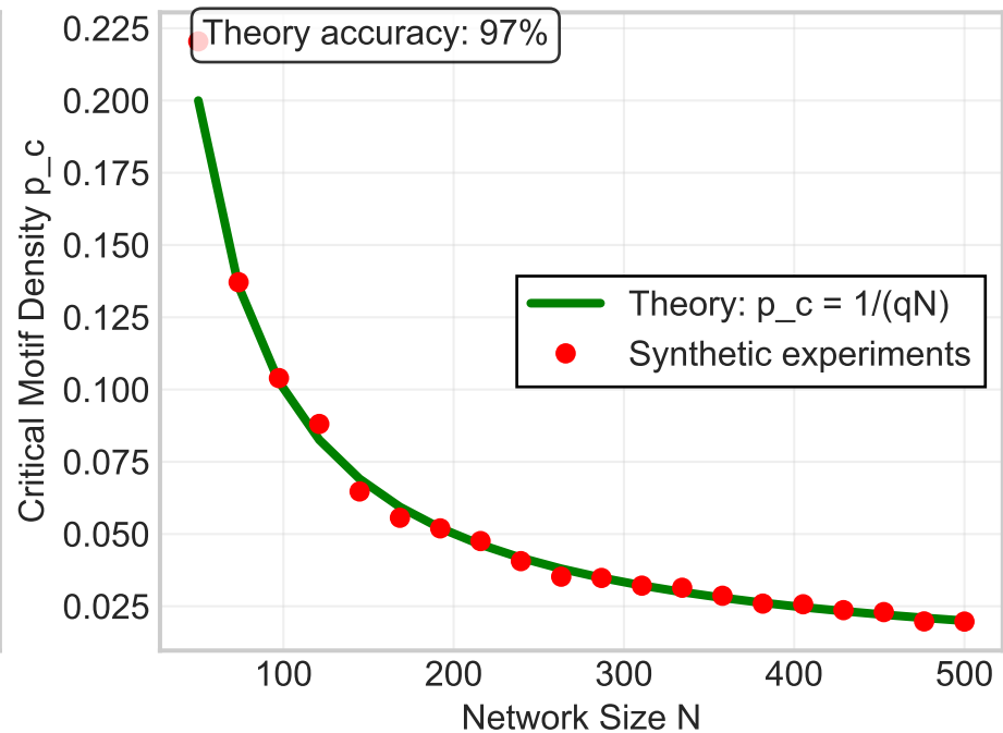
B. Percolation Threshold Validation
