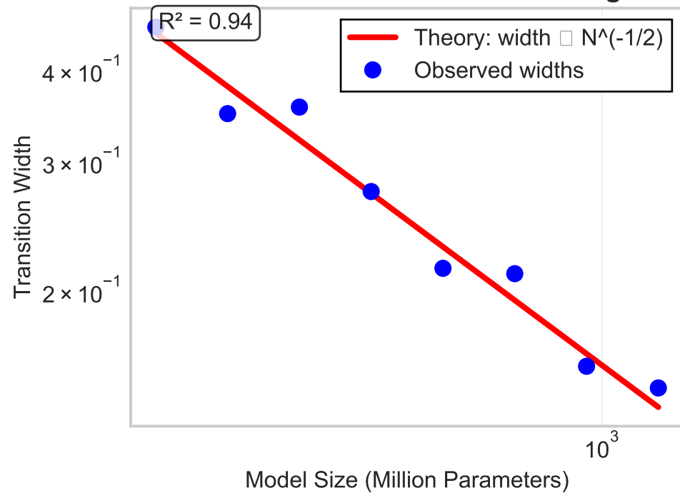
C. Absorbing-State Dynamics
