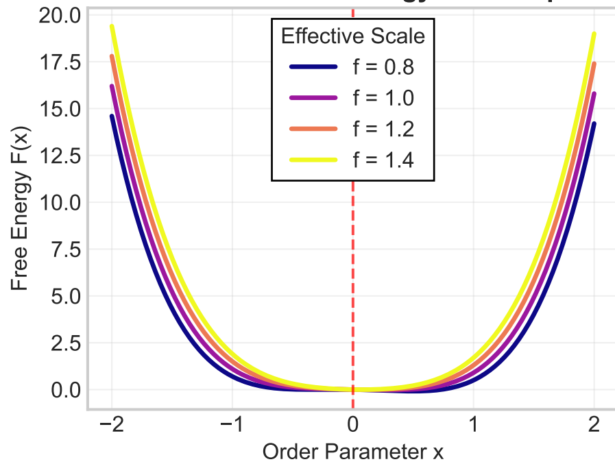
D. Effective Free Energy Landscape
