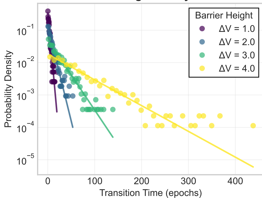
C. Absorbing-State Dynamics
