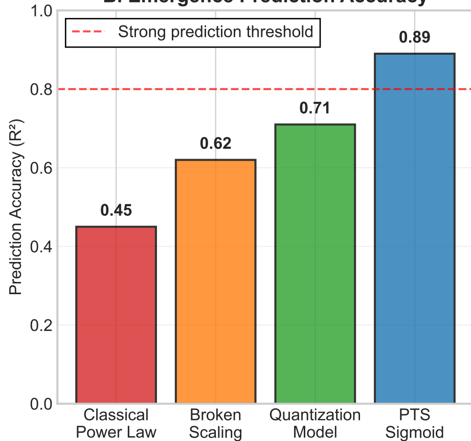
B. Emergence Prediction Accuracy
