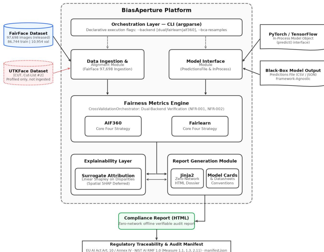
Figure 4-1. BiasAperture system architecture.
