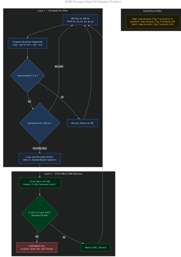
Figure 5.2: Two-layer fall detection flowchart: Layer 1 threshold pre-filter (top zone) gates Layer 2 TFLite Micro CNN inference (bottom zone). Sensitivity profile thresholds are shown in the callout.
