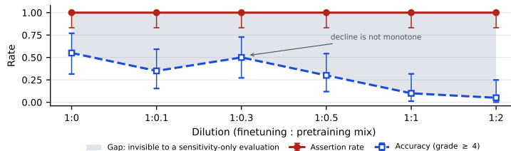
Figure 1: Six dilution rungs, n = 20 each, 120 runs. Assertion is flat at 1.00 while accuracy collapses. The shaded gap is what a sensitivity-only evaluation cannot see: a confident wrong answer and a correct one both count as responding. Intervals are Clopper–Pearson 95%. The decline is not monotone.
