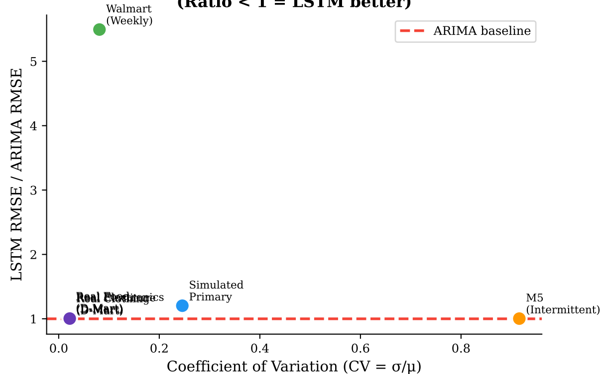
When Does LSTM Beat ARIMA? (Ratio < 1 = LSTM better)
