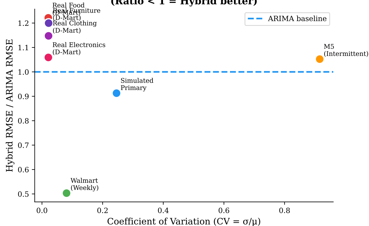
When Does Hybrid Beat ARIMA? (Ratio < 1 = Hybrid better)
