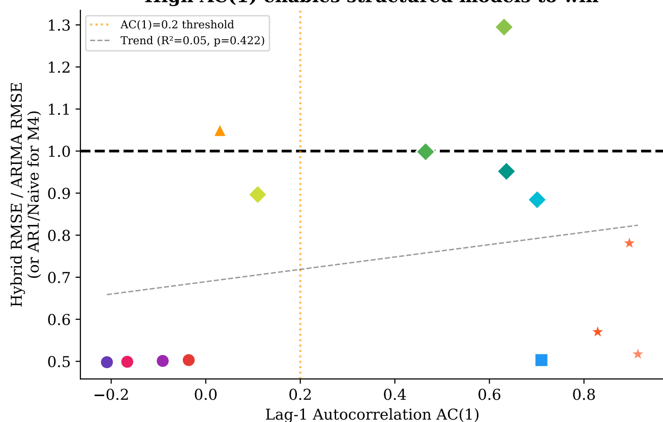
AC(1) vs Model Performance High AC(1) enables structured models to win
