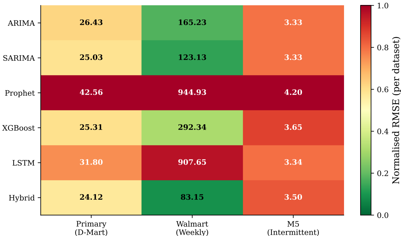
RMSE Comparison Across Models and Datasets
