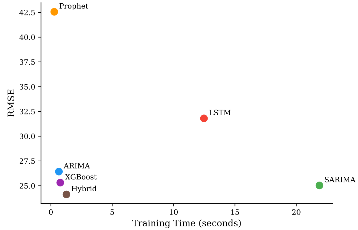
Accuracy-Efficiency Trade-off (Primary Dataset)
