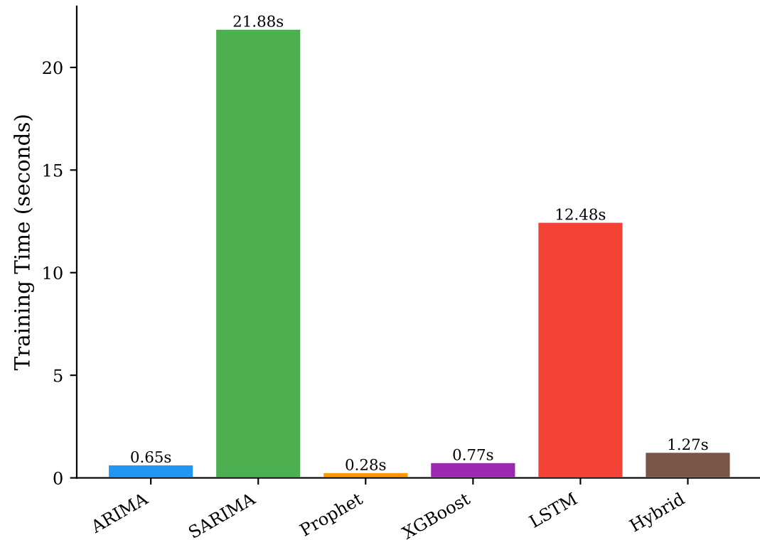
Computational Cost (Primary Dataset)
