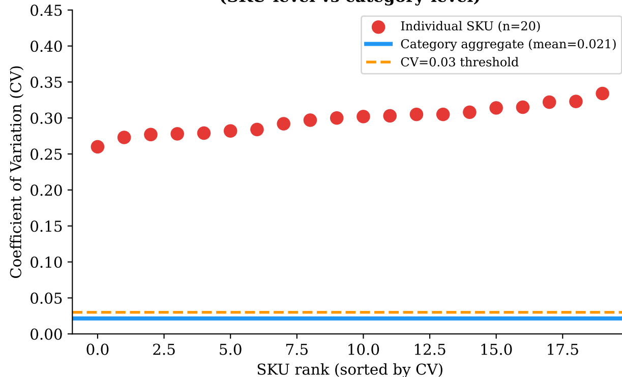
Aggregation Reduces CV by ~14× (SKU-level vs category-level)
