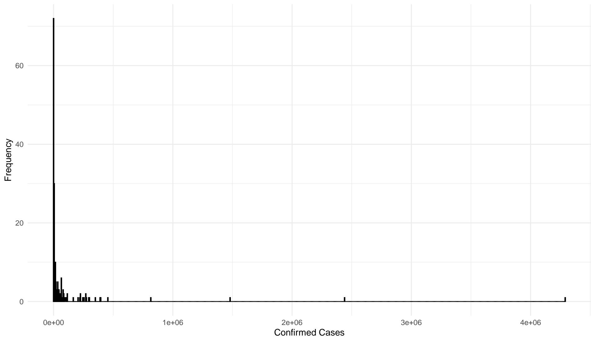
Histogram of Confirmed Cases
