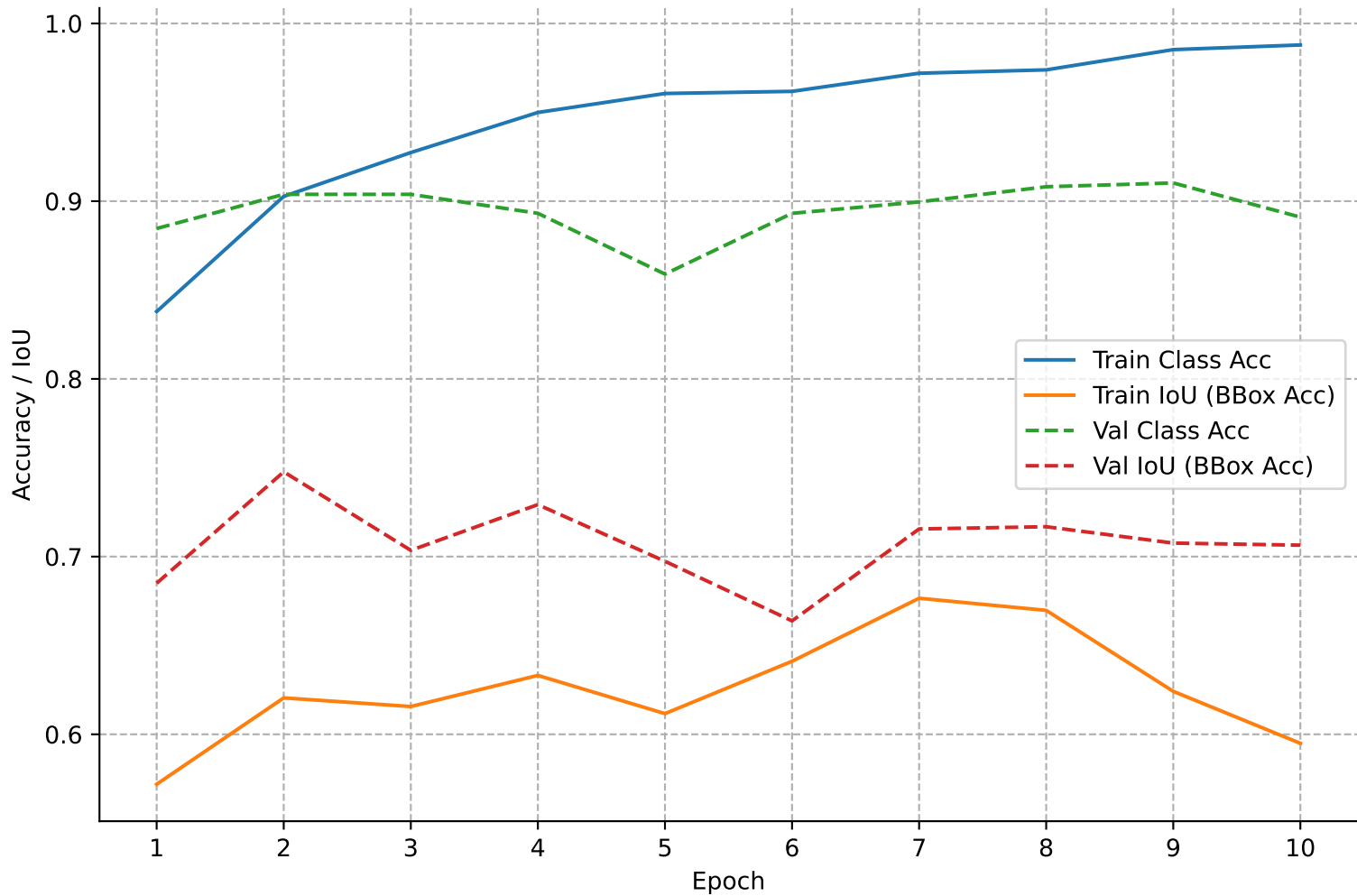
Accuracy Metrics
