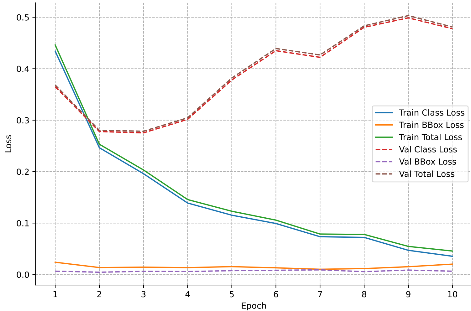
Loss Metrics
