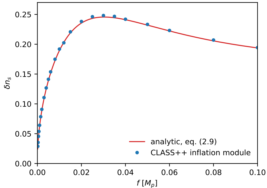
Flauger et al. fig. 1 ( b = 0.08 )
