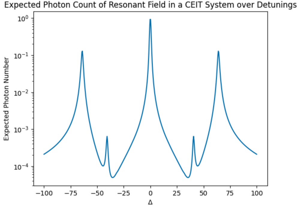
FIG. 13: Reproduction of a portion of figure 1(c) from ‘Coherent Control of Quantum Fluctuations Using Cavity Electromagnetically Induced Transparency’ by Souza et al. [42] depicting the expected photon count within the cavity over a range of frequency detunings \Delta .
