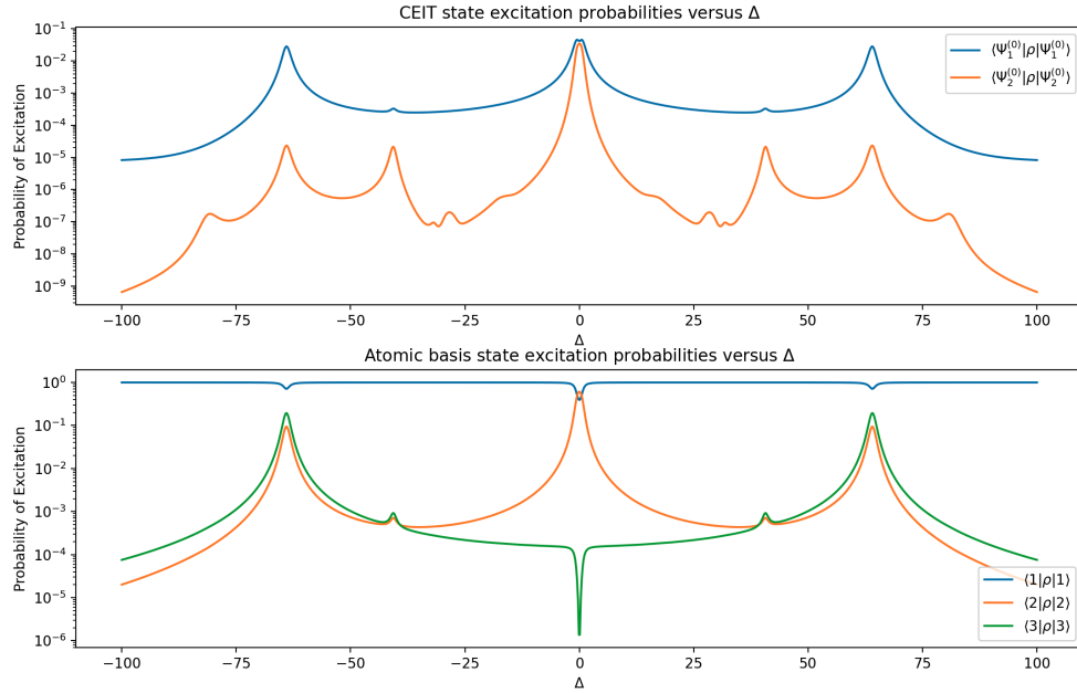
FIG. 14: Reproduction of a portion of figure 1(c) from ‘Coherent Control of Quantum Fluctuations Using Cavity Electromagnetically Induced Transparency’ by Souza et al. [42] — which has been slightly modified and added upon for clarity — depicting (top) the state expectation values of states in an energy split and rotated basis over a range of detunings and (bottom) the state expectation values of states in the atomic basis over a range of detunings.
