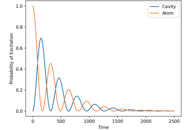
Rabi Oscillation in Jaynes-Cummings Model
