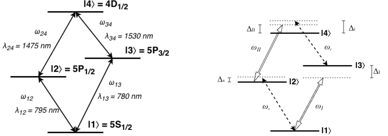
FIG. 15: Diamond configuration atom diagrams. (Left) Duplicate of Fig. ?? placed for convenience. A diamond configuration atomic system with non-degenerate energy levels |1\rangle, |2\rangle, |3\rangle, |4\rangle . The system has allowed transitions |1\rangle \leftrightarrow |2\rangle , |1\rangle \leftrightarrow |3\rangle , |2\rangle \leftrightarrow |4\rangle , and |3\rangle \leftrightarrow |4\rangle with respective energies \hbar\omega_{12} , \hbar\omega_{13} , \hbar\omega_{24} , and \hbar\omega_{34} and corresponding wavelengths \lambda_{12} , \lambda_{13} , \lambda_{24} , and \lambda_{34} . (Right) A strong pump drives transition |1\rangle \leftrightarrow |3\rangle at frequency \omega_I with detuning \Delta_I = \omega_I - \omega_{13} , a separate strong pump drives transition |2\rangle \leftrightarrow |4\rangle with detuning \Delta_{II} = \omega_{II} - \omega_{24} , a weak signal beam drives transition |1\rangle \leftrightarrow |2\rangle with detuning \Delta_s = \omega_s - \omega_{12} , and a weak idler field (undriven) is induced by the presence of the other fields through a FWM process, resulting in transition |3\rangle \leftrightarrow |4\rangle with emission detuning \Delta_i = \omega_i - \omega_{34} .
