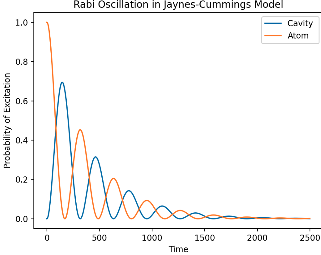
FIG. 10: Decaying Rabi oscillation produced by the Jaynes-Cummings model with initial state |\psi\rangle_0 = |e\rangle \otimes |0\rangle .
