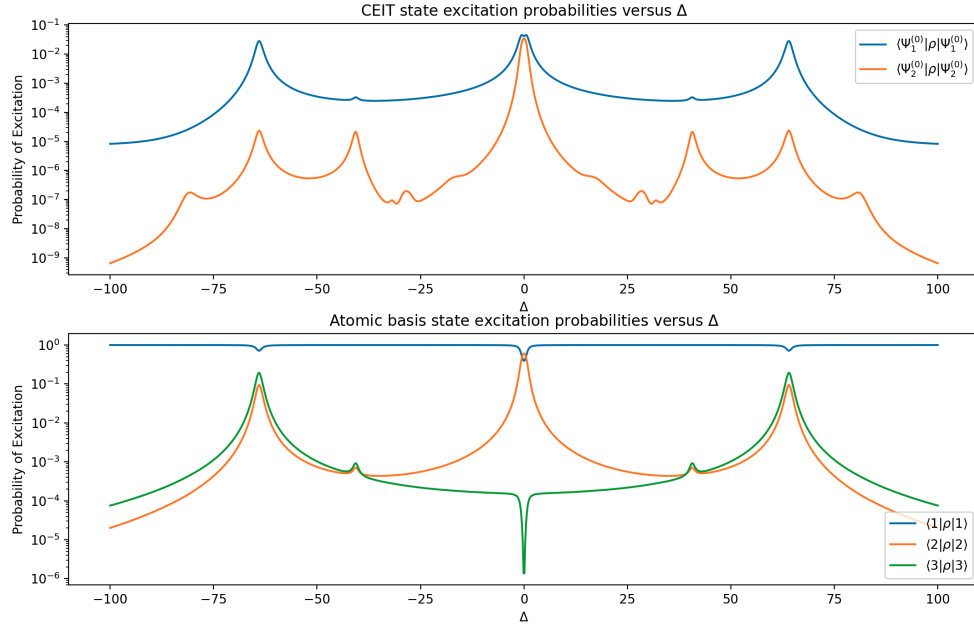
FIG. 14: Reproduction of a portion of figure 1(c) from ‘Coherent Control of Quantum Fluctuations Using Cavity Electromagnetically Induced Transparency’ by Souza et al. [?] — which has been slightly modified and added upon for clarity — depicting (top) the state expectation values of states in an energy split and rotated basis over a range of detunings and (bottom) the state expectation values of states in the atomic basis over a range of detunings.
