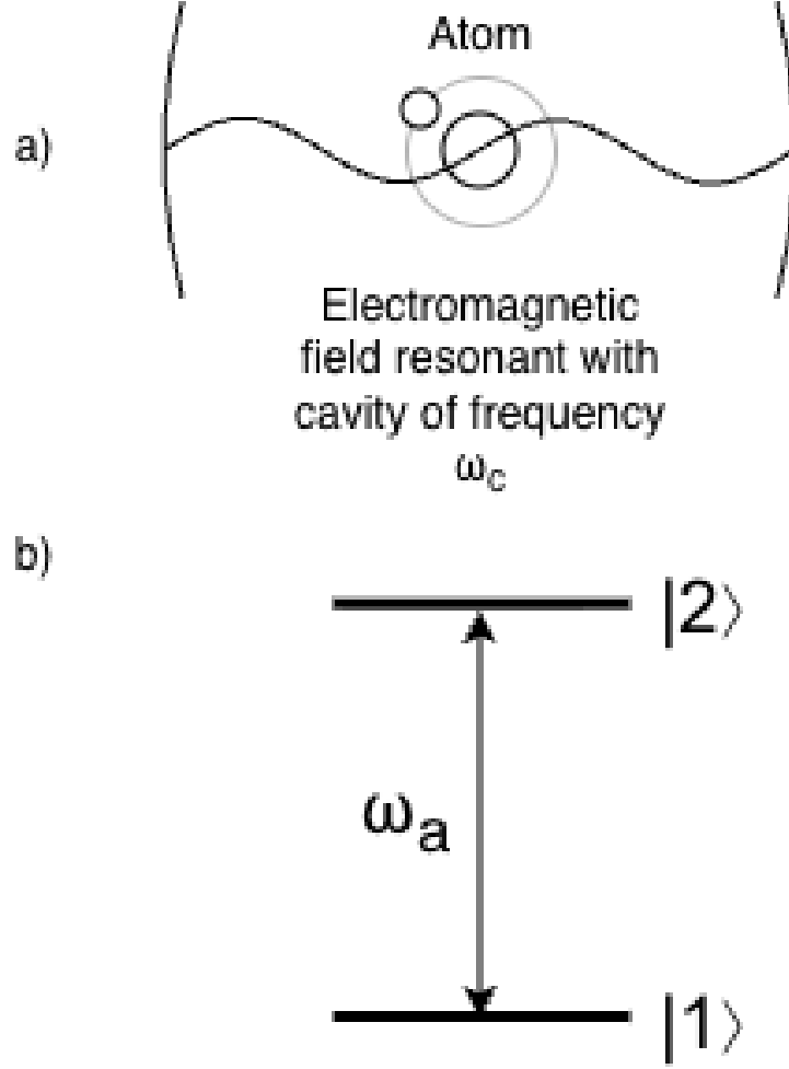
FIG. 5: Depiction of the system for a Jaynes-Cummings model with (a) a resonant cavity of frequency \omega_c containing (b) a two-level atom of transition frequency \omega_a .
