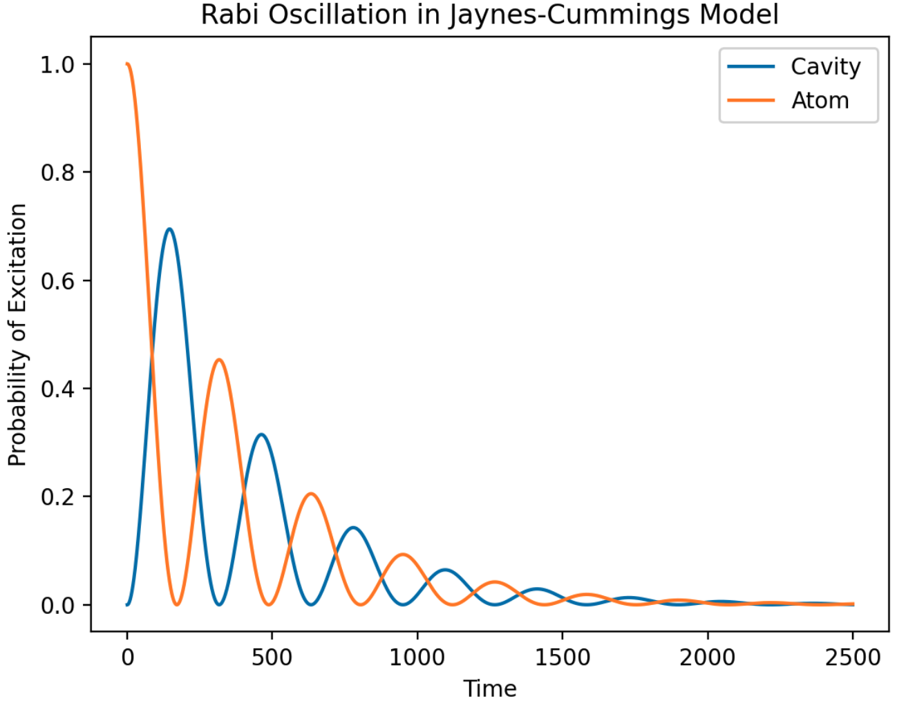
FIG. 9: Decaying Rabi oscillation produced by the Jaynes-Cummings model with initial state |\psi\rangle_0 = |e\rangle \otimes |0\rangle .
