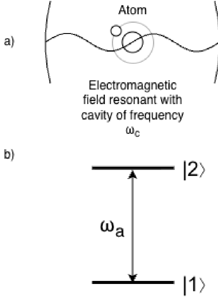
FIG. 8: Depiction of the system for a Jaynes-Cummings model with (a) a resonant cavity of frequency \omega_c containing (b) a two-level atom of transition frequency \omega_a .
