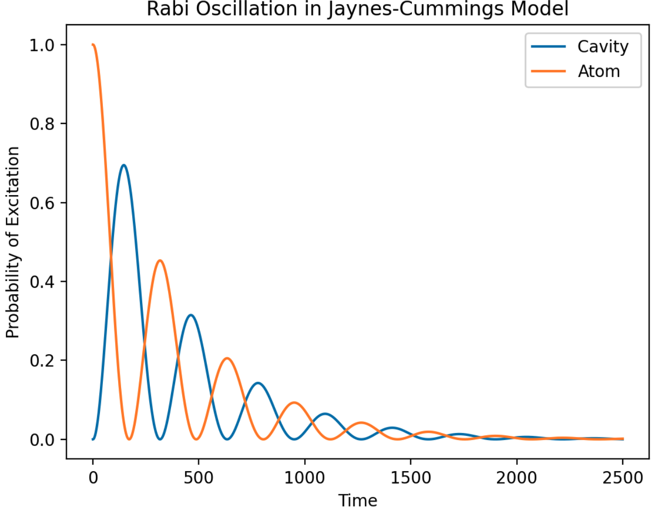
FIG. 4: Decaying Rabi oscillation produced by the Jaynes-Cummings model with initial state |\psi\rangle_0 = |e\rangle \otimes |0\rangle .
