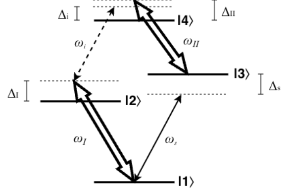
(b) A strong pump drives transition |1\rangle \leftrightarrow |2\rangle at frequency \omega_I with detuning \Delta_I = \omega_I - \omega_{12} , a separate strong pump drives transition |3\rangle \leftrightarrow |4\rangle with detuning \Delta_{II} = \omega_{II} - \omega_{34} , a weak signal beam drives transition |1\rangle \leftrightarrow |3\rangle with detuning \Delta_s = \omega_s - \omega_{13} , and a weak idler beam drives transition |2\rangle \leftrightarrow |4\rangle with detuning \Delta_i = \omega_i - \omega_{24} .
