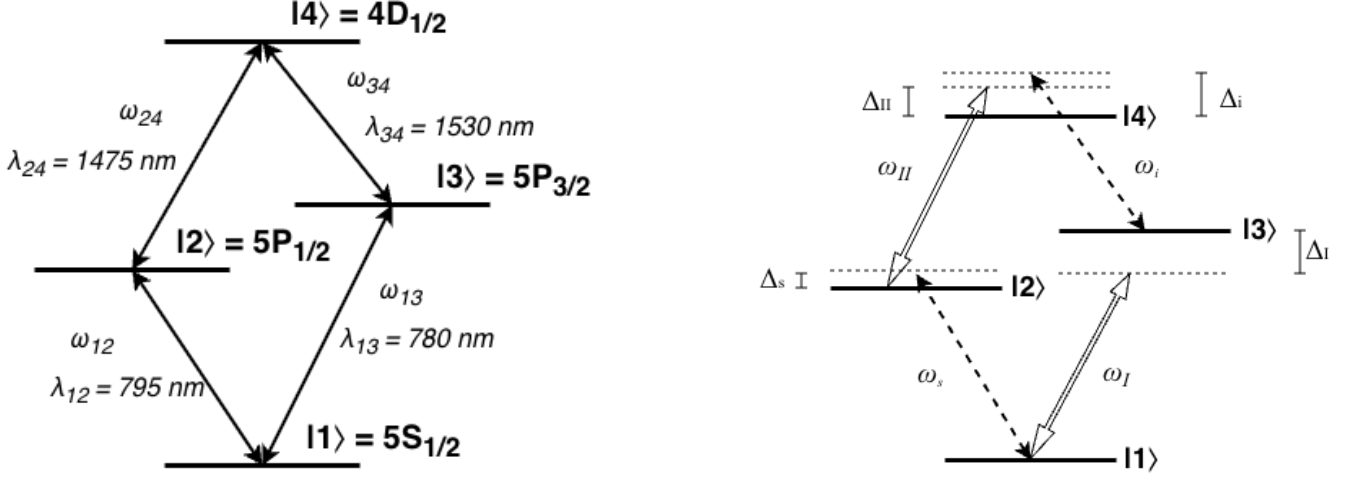
FIG. 15: Diamond configuration atom diagrams. (Left) Duplicate of Fig. 3 placed for convenience. A diamond configuration atomic system with non-degenerate energy levels |1\rangle, |2\rangle, |3\rangle, |4\rangle . The system has allowed transitions |1\rangle \leftrightarrow |2\rangle , |1\rangle \leftrightarrow |3\rangle , |2\rangle \leftrightarrow |4\rangle , and |3\rangle \leftrightarrow |4\rangle with respective energies \hbar\omega_{12} , \hbar\omega_{13} , \hbar\omega_{24} , and \hbar\omega_{34} and corresponding wavelengths \lambda_{12} , \lambda_{13} , \lambda_{24} , and \lambda_{34} . (Right) A strong pump drives transition |1\rangle \leftrightarrow |3\rangle at frequency \omega_I with detuning \Delta_I = \omega_I - \omega_{13} , a separate strong pump drives transition |2\rangle \leftrightarrow |4\rangle with detuning \Delta_{II} = \omega_{II} - \omega_{24} , a weak signal beam drives transition |1\rangle \leftrightarrow |2\rangle with detuning \Delta_s = \omega_s - \omega_{12} , and a weak idler field (undriven) is induced by the presence of the other fields through a FWM process, resulting in transition |3\rangle \leftrightarrow |4\rangle with emission detuning \Delta_i = \omega_i - \omega_{34} .
