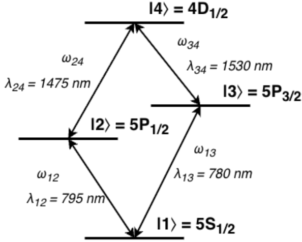
(a) Duplicate of Fig. ??? placed for convenience. A diamond configuration atomic system with non-degenerate energy levels |1\rangle, |2\rangle, |3\rangle, |4\rangle . The system has allowed transitions |1\rangle \leftrightarrow |2\rangle , |1\rangle \leftrightarrow |3\rangle , |2\rangle \leftrightarrow |4\rangle , and |3\rangle \leftrightarrow |4\rangle with respective energies \hbar\omega_{12} , \hbar\omega_{13} , \hbar\omega_{24} , and \hbar\omega_{34} and corresponding wavelengths \lambda_{12} , \lambda_{13} , \lambda_{24} , and \lambda_{34} .
