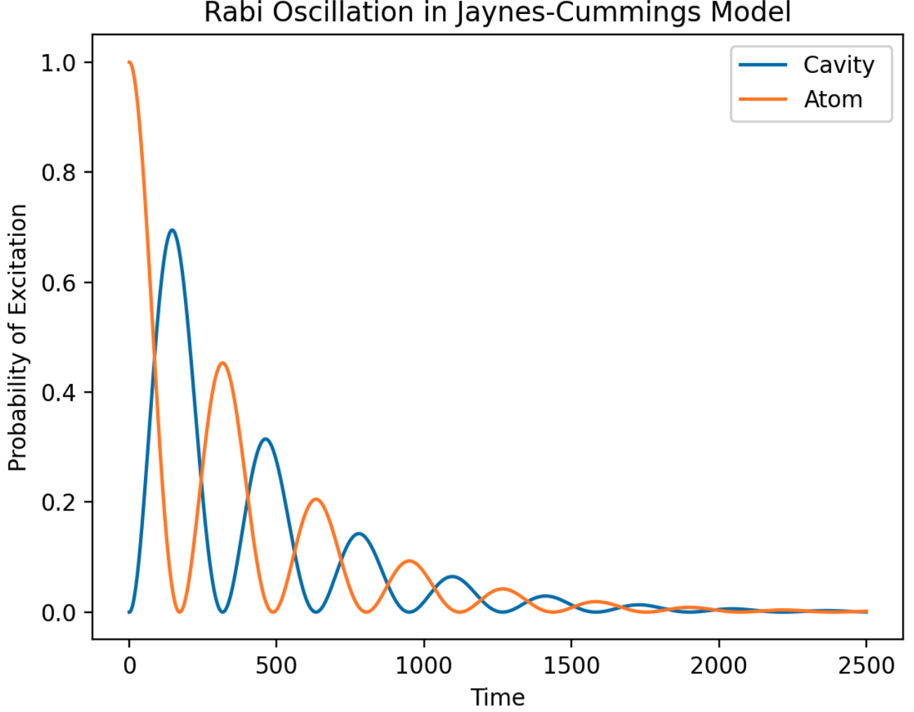
FIG. 5: Decaying Rabi oscillation produced by the Jaynes-Cummings model with initial state |\psi\rangle_0 = |e\rangle \otimes |0\rangle .
