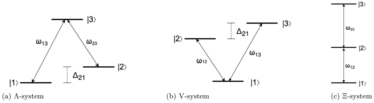
FIG. 1: Three-level atomic configurations: (a) \Lambda , (b) V , and (c) \Xi systems.
