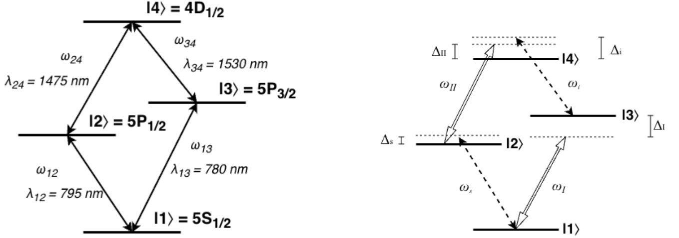
FIG. 11: Diamond configuration atom diagrams. (Left) Duplicate of Fig. ??? placed for convenience. A diamond configuration atomic system with non-degenerate energy levels |1\rangle, |2\rangle, |3\rangle, |4\rangle . The system has allowed transitions |1\rangle \leftrightarrow |2\rangle , |1\rangle \leftrightarrow |3\rangle , |2\rangle \leftrightarrow |4\rangle , and |3\rangle \leftrightarrow |4\rangle with respective energies \hbar\omega_{12} , \hbar\omega_{13} , \hbar\omega_{24} , and \hbar\omega_{34} and corresponding wavelengths \lambda_{12} , \lambda_{13} , \lambda_{24} , and \lambda_{34} . (Right) A strong pump drives transition |1\rangle \leftrightarrow |3\rangle at frequency \omega_I with detuning \Delta_I = \omega_I - \omega_{13} , a separate strong pump drives transition |2\rangle \leftrightarrow |4\rangle with detuning \Delta_{II} = \omega_{II} - \omega_{24} , a weak signal beam drives transition |1\rangle \leftrightarrow |2\rangle with detuning \Delta_s = \omega_s - \omega_{12} , and a weak idler field (undriven) is induced by the presence of the other fields through a FWM process, resulting in transition |3\rangle \leftrightarrow |4\rangle with emission detuning \Delta_i = \omega_i - \omega_{34} .
