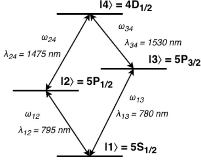
FIG. 3: A diamond configuration atomic system with non-degenerate energy levels |1\rangle, |2\rangle, |3\rangle, |4\rangle . The system has allowed transitions |1\rangle \leftrightarrow |2\rangle , |1\rangle \leftrightarrow |3\rangle , |2\rangle \leftrightarrow |4\rangle , and |3\rangle \leftrightarrow |4\rangle with respective energies \hbar\omega_{12} , \hbar\omega_{13} , \hbar\omega_{24} , and \hbar\omega_{34} and corresponding wavelengths \lambda_{12} , \lambda_{13} , \lambda_{24} , and \lambda_{34} .
