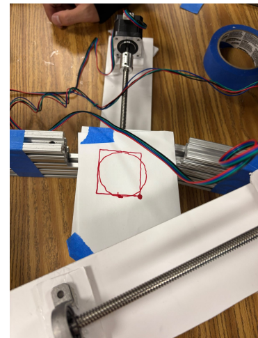
Early path test; rounded corners and line waviness remain visible.
