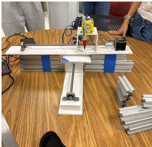
Preliminary Cartesian test rig used before the fishing-game mechanism.
