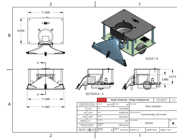
Assembly drawing showing packaging and service access.
