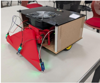
Prototype used for presentation and pickup testing.
