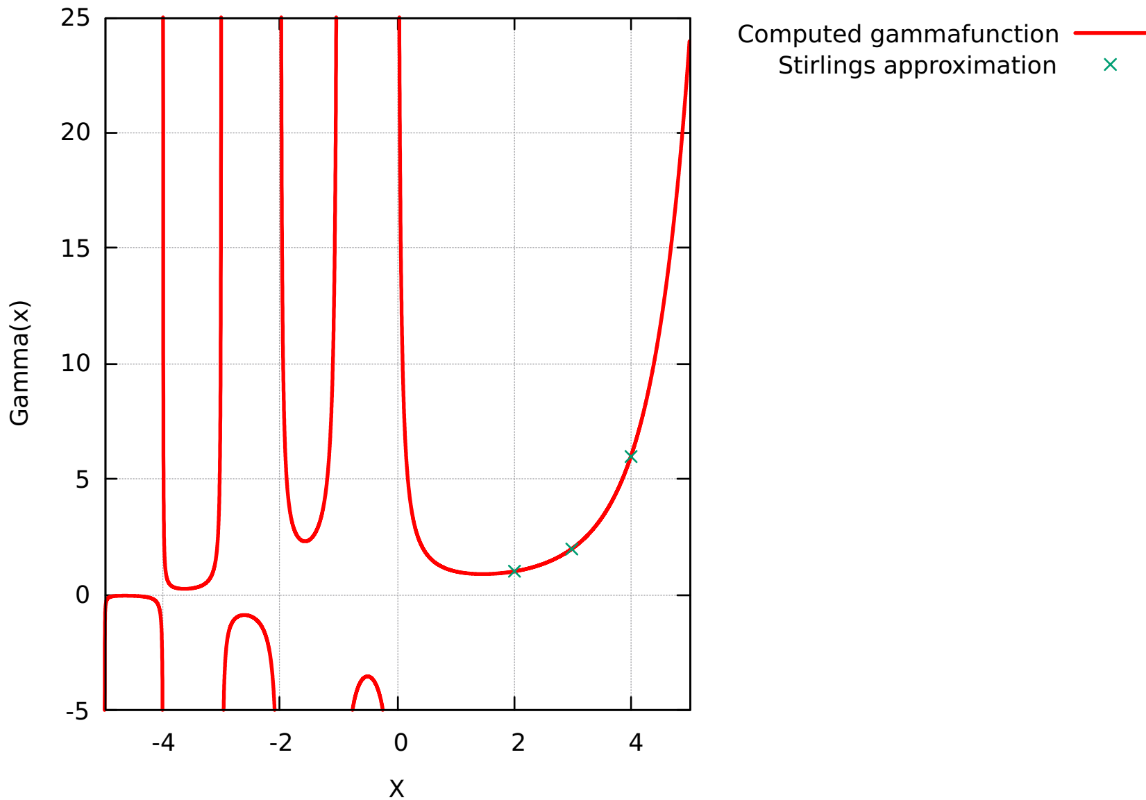
gamma function
