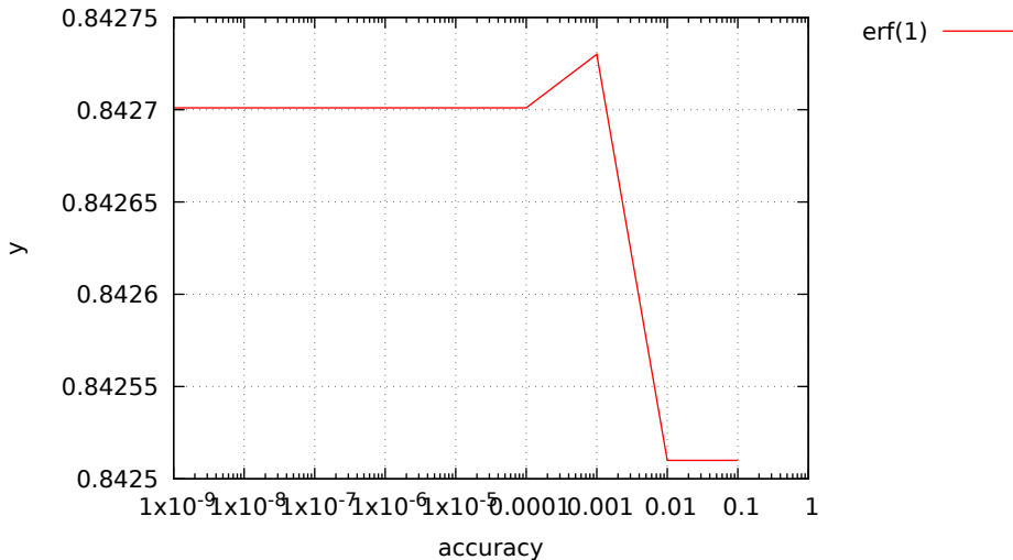
Evaluating erf(1) with numeric integration
