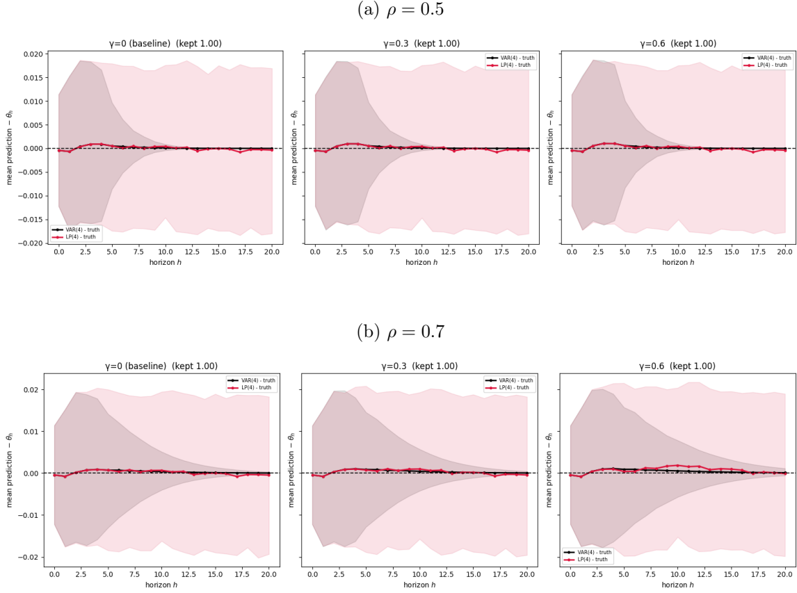
Figure 6: Asymptotic Deviation from the True IRF
