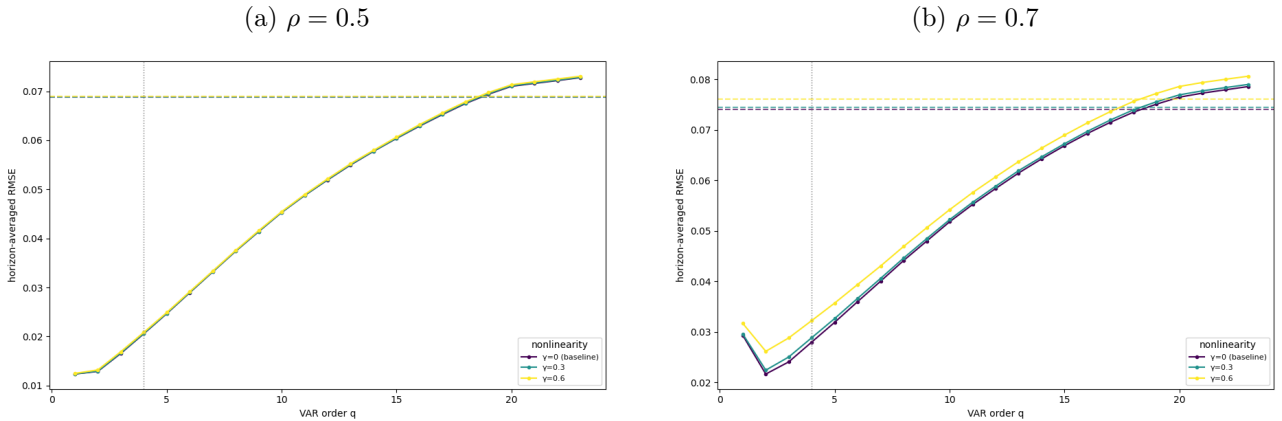
Figure 7: Complexity Frontier under Nonlinear Lag Misspecification
