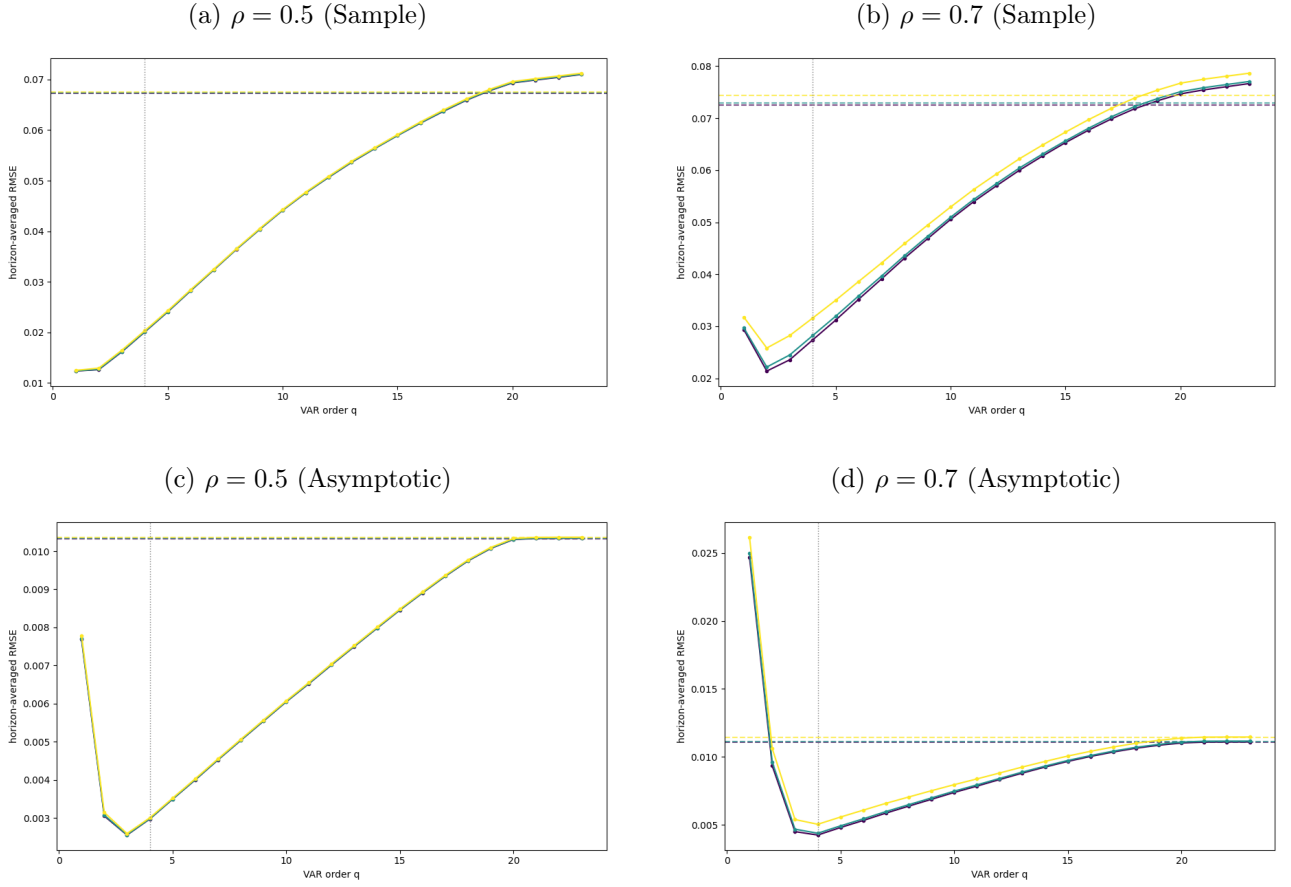
Figure 10: Complexity Frontier under Nonlinear Lag Misspecification
