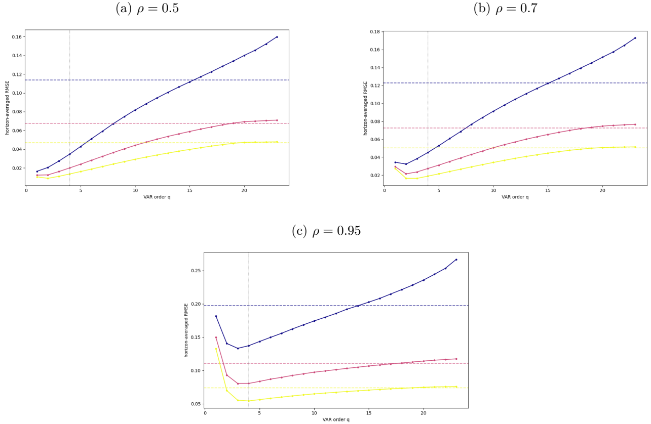
Figure 2: Complexity Frontier Across Persistence Regimes
