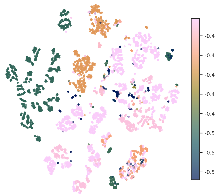
MinPartialCharge
