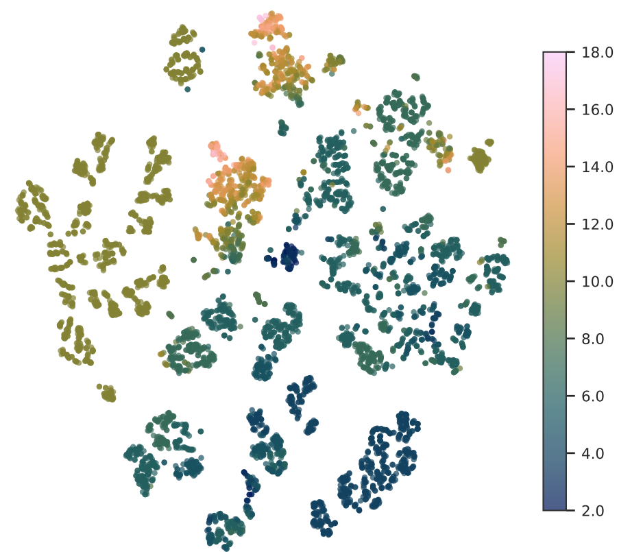
Nchiral
