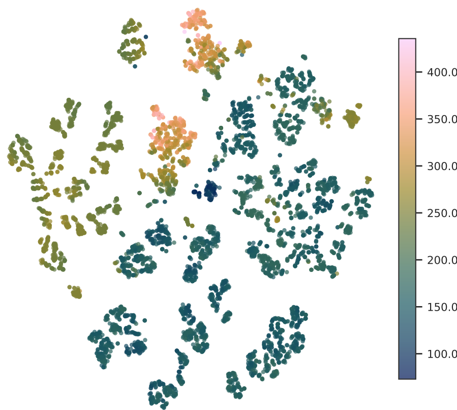
TPSA
