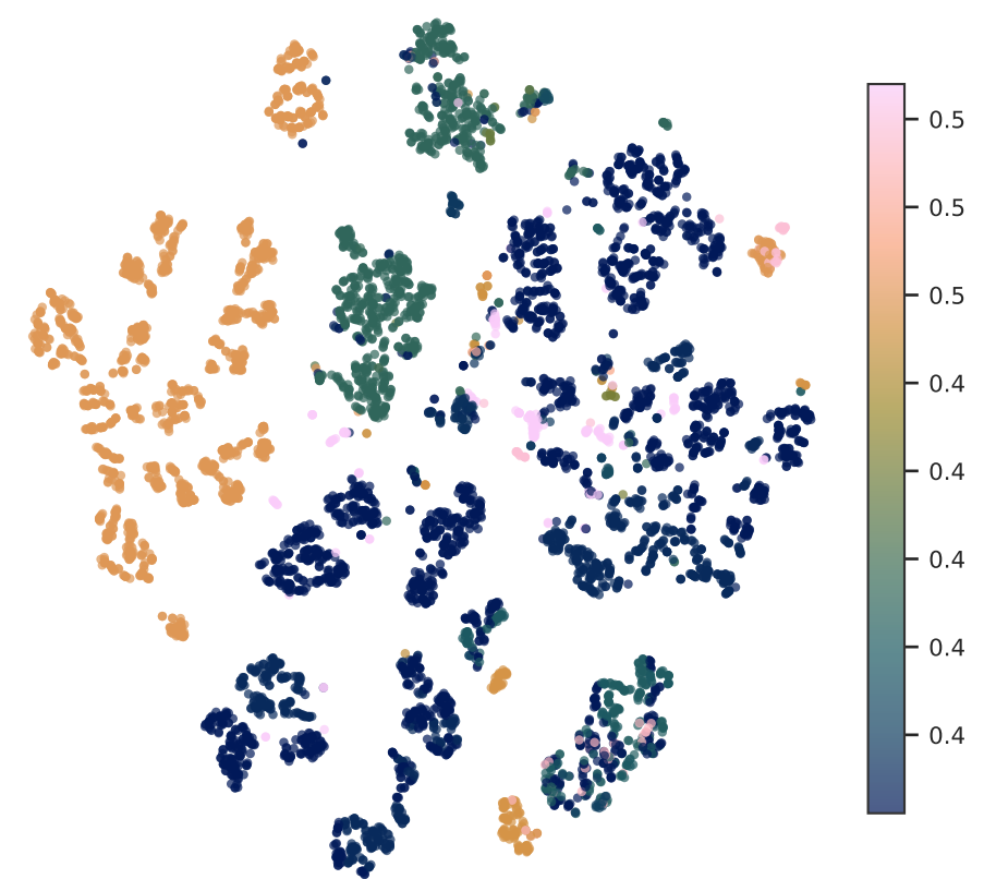
MaxAbsPartialCharge
