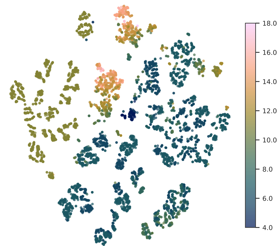
NumHAcceptors
