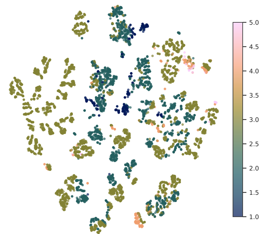
NumAliphaticRings
