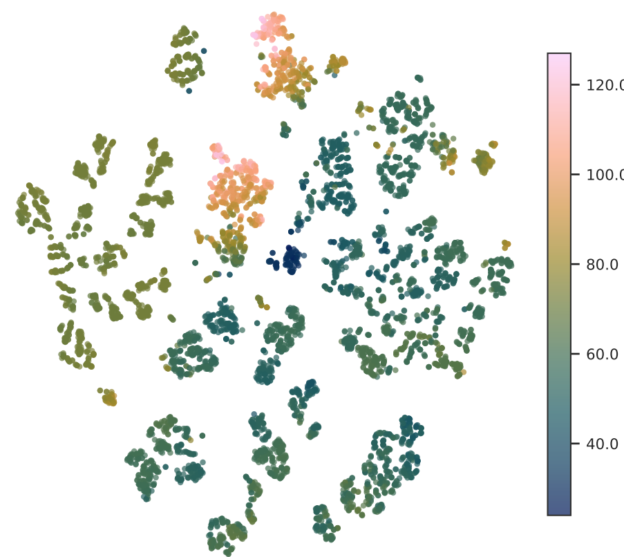
Num_Atoms
