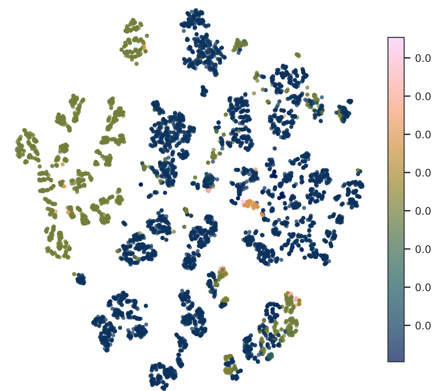
MinAbsPartialCharge
