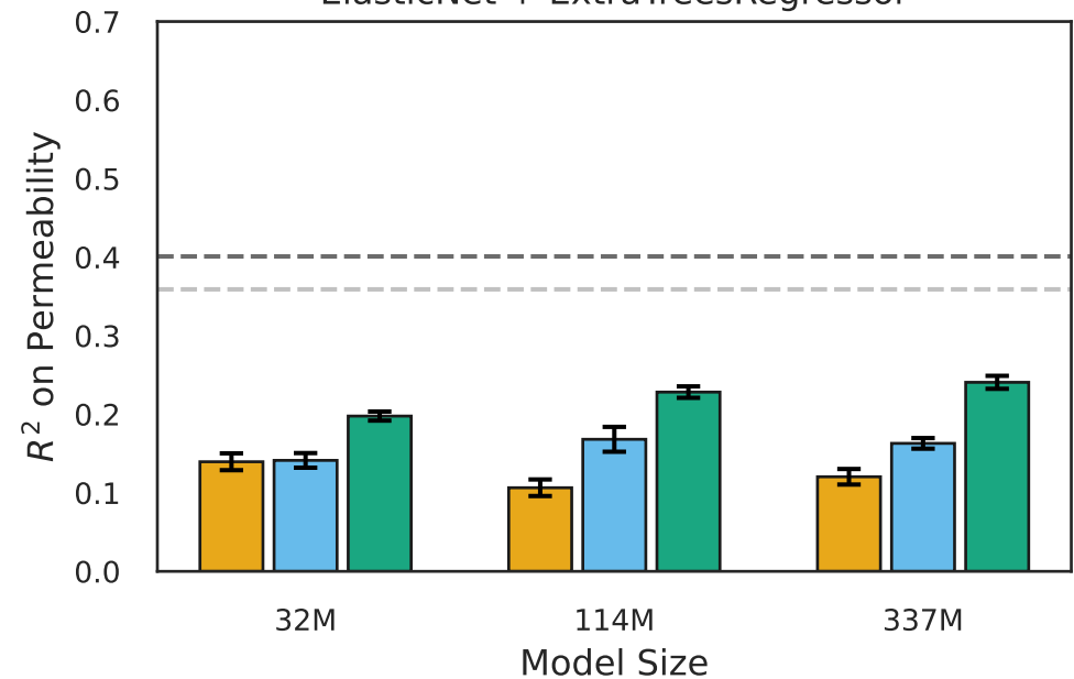
ElasticNet + ExtraTreesRegressor
