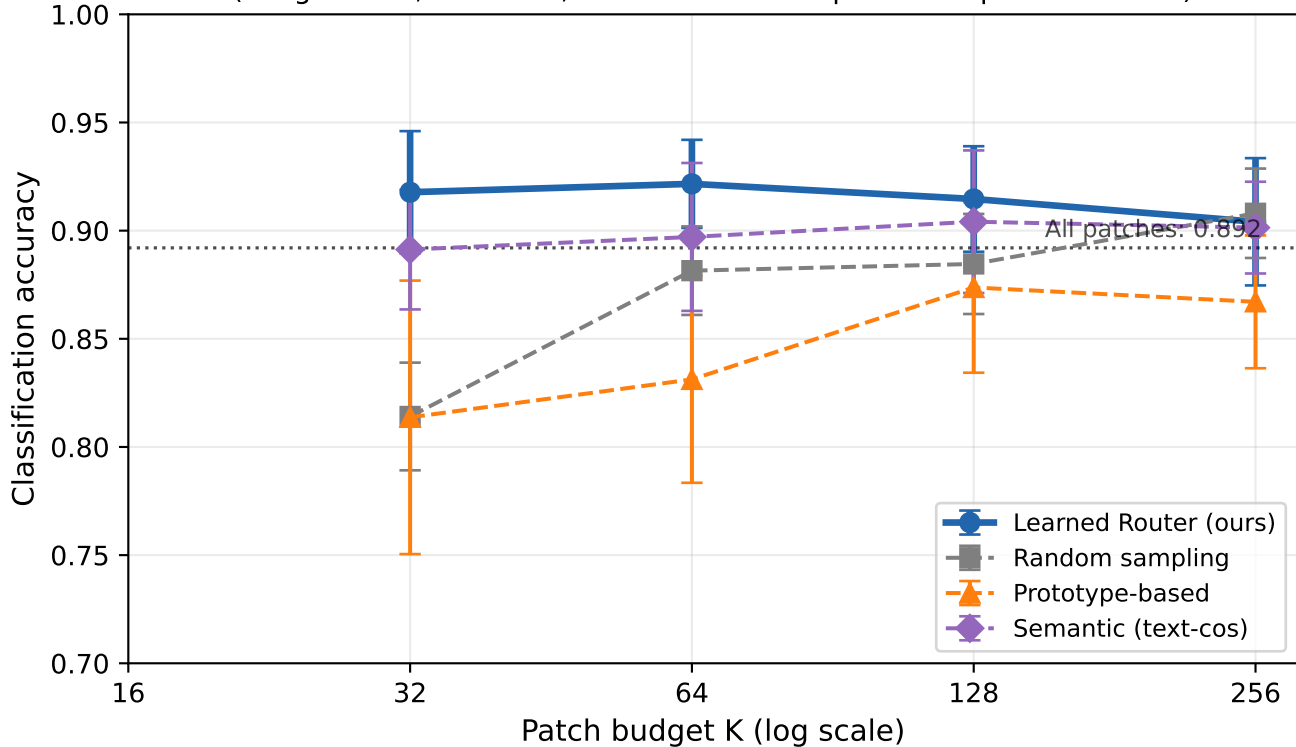
Budget Efficiency: Patch Selection Strategy vs. Accuracy (Lung cancer, 3-fold CV; learned router surpasses all-patch at K=64)
