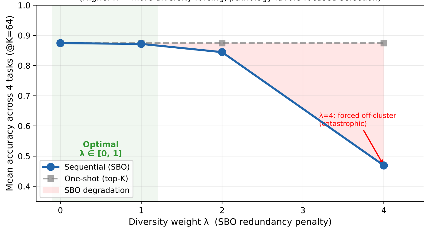
Sequential Budgeted Observer: \lambda vs. Accuracy (Higher \lambda = more diversity forcing; pathology favors focused selection)
