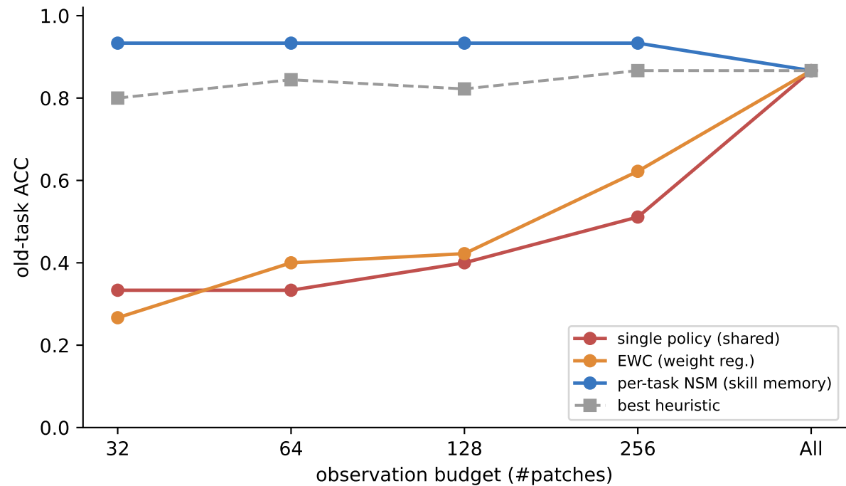
Navigation forgetting vs budget (old ESCA, reverse order)
