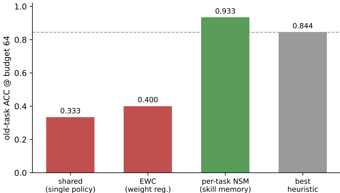
Which continual mechanism fits a WSI navigation policy? (old ESCA, reverse order, mean over folds)
