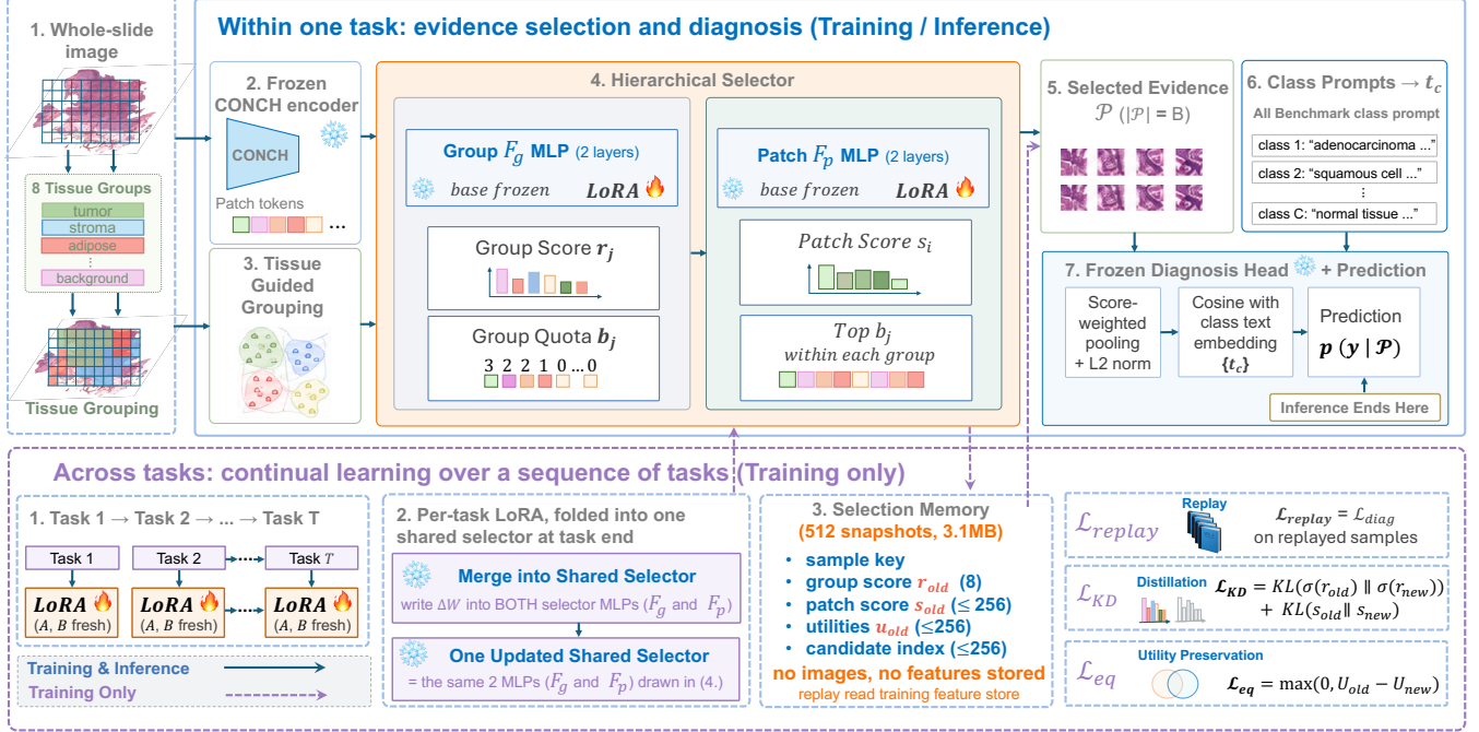
Fig. 1. PathSelect overview. Top (solid arrows; training and inference): frozen CONCH patch features are grouped by eight fixed tissue prompts; the group selector F_g turns group scores into integer quotas ( \sum_j b_j = B = 8 ), the patch selector F_p keeps the top b_j patches within each group, and the frozen head diagnoses from the selected evidence alone by cosine with the class-text embeddings—inference ends there. Bottom (dashed; training only): each task trains fresh LoRA adapters on the same two MLPs and folds them into one shared selector at the task end; a Selection Memory of 512 behavioral snapshots (scores, indices, utilities; no images or features) drives replay, dual-level distillation, and the utility-preservation hinge.
