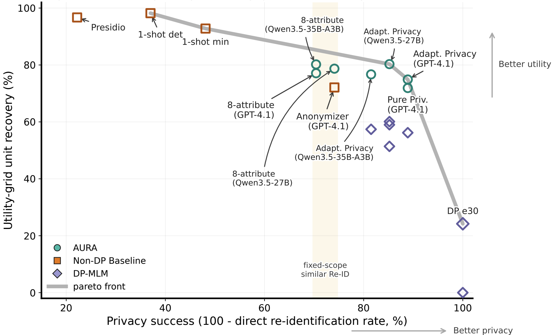
pareto front for privacy vs. utility-grid unit recovery (GPT-5.4-mini)
