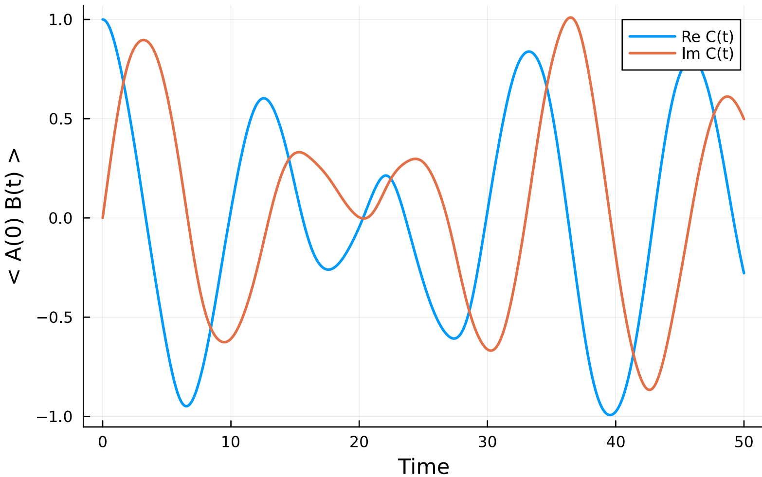
Correlation function: H2_6-31g
