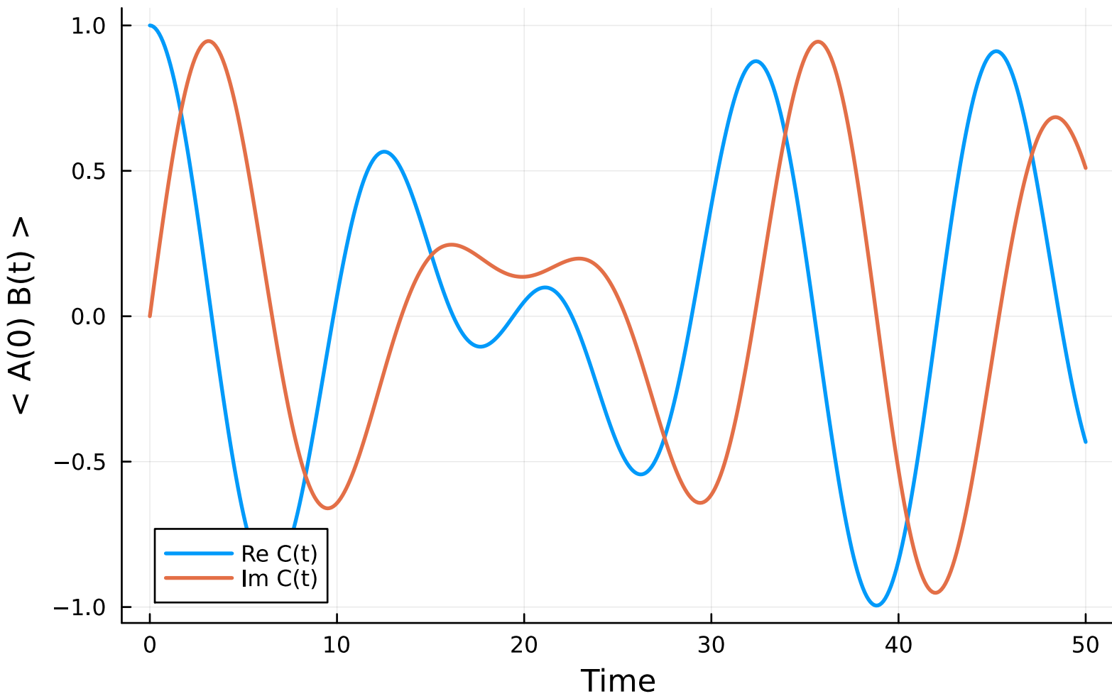
Correlation function: H2_AS_2_2_6-31g
