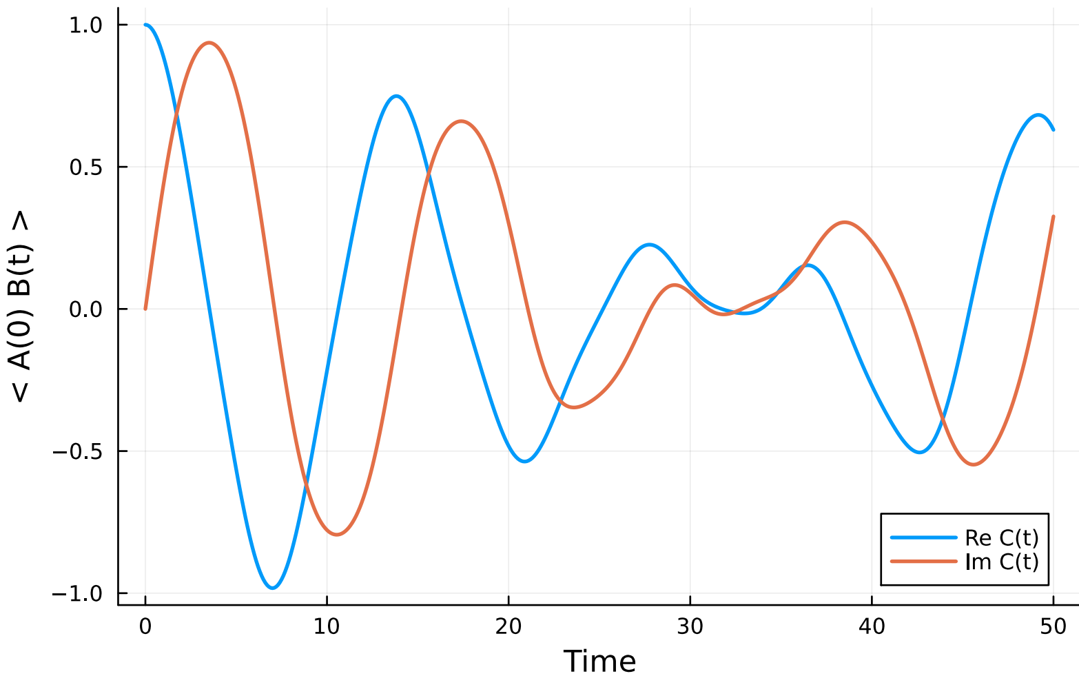
Correlation function: H2_AS_3_2_ccpvdz
