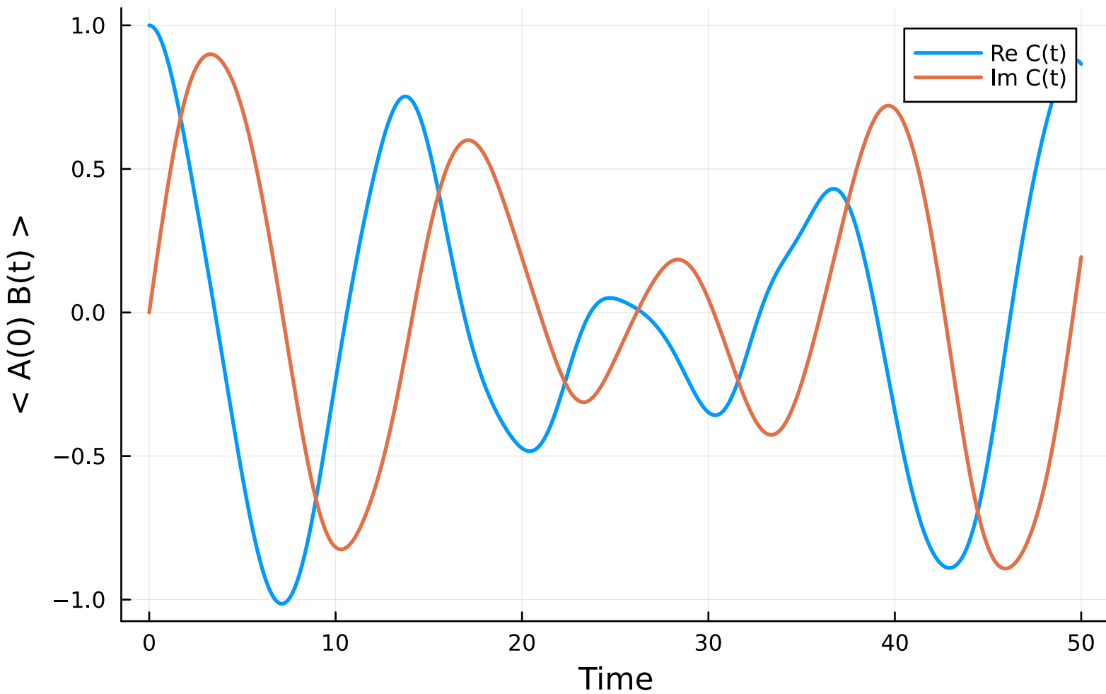
Correlation function: H2_AS_4_2_ccpvdz
