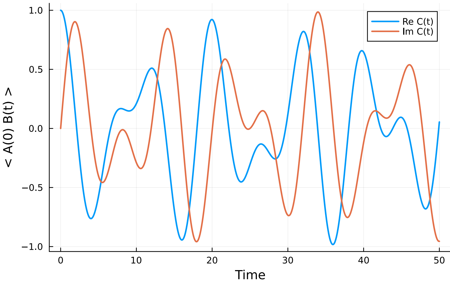
Correlation function: H2_sto3g
