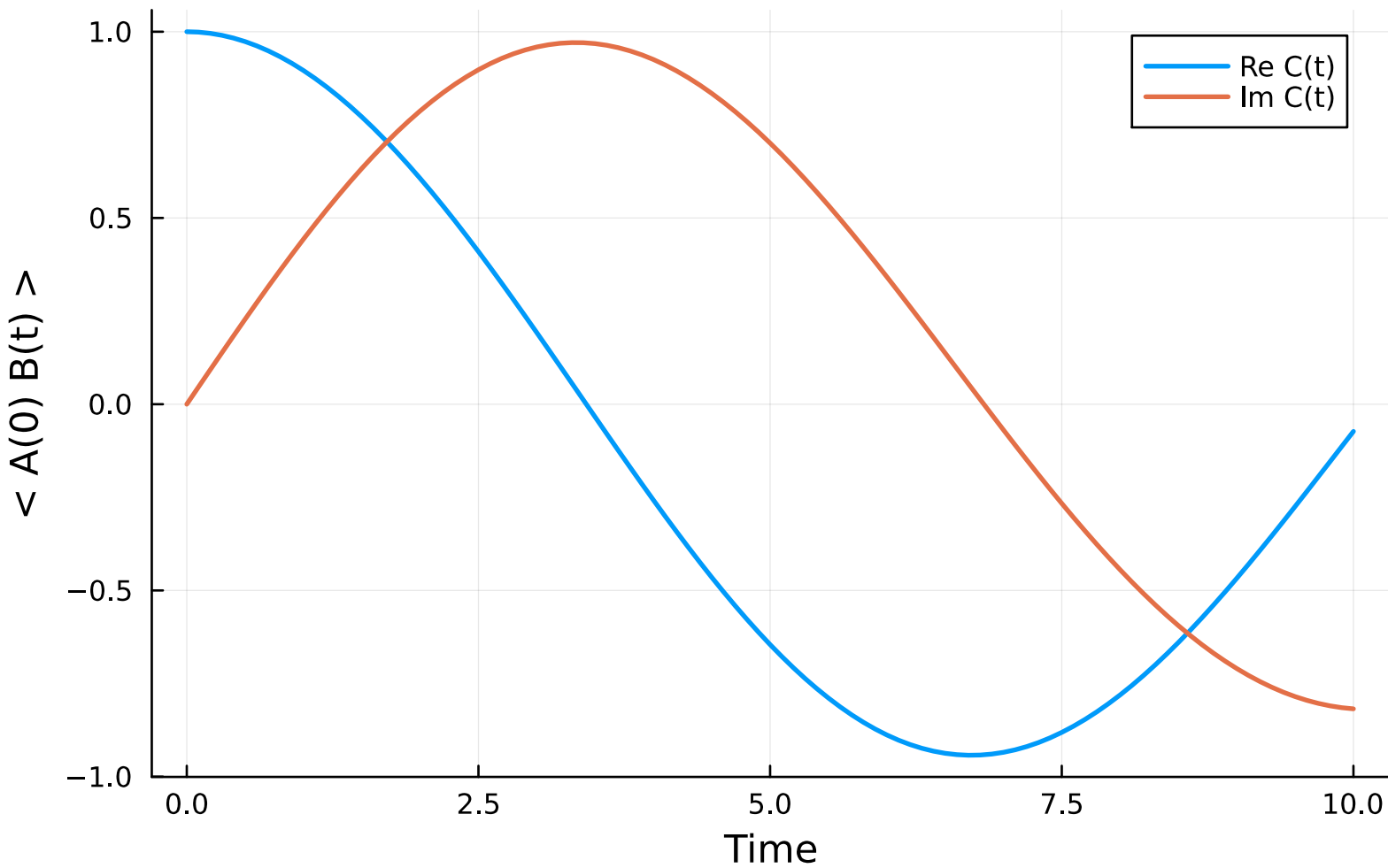
Correlation function: H2_AS_2_2_ccpvdz
