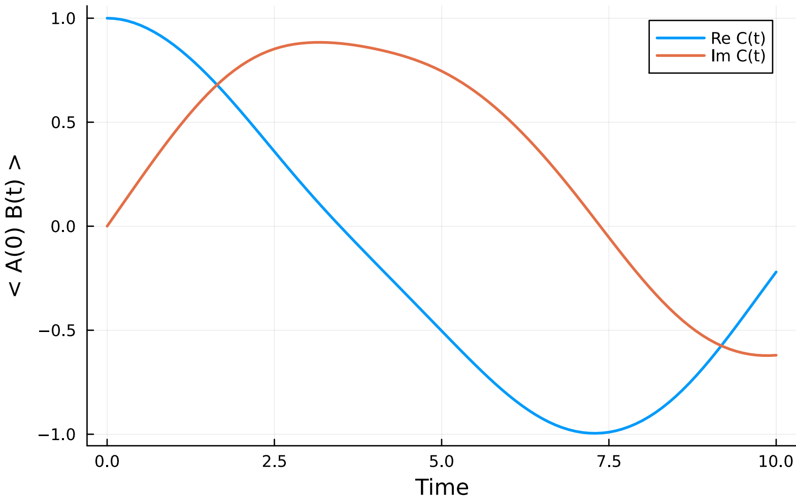
Correlation function: H2_AS_5_2_ccpvdz
