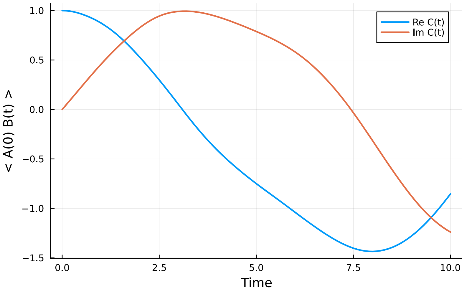
Correlation function: H2_AS_6_2_ccpvdz
