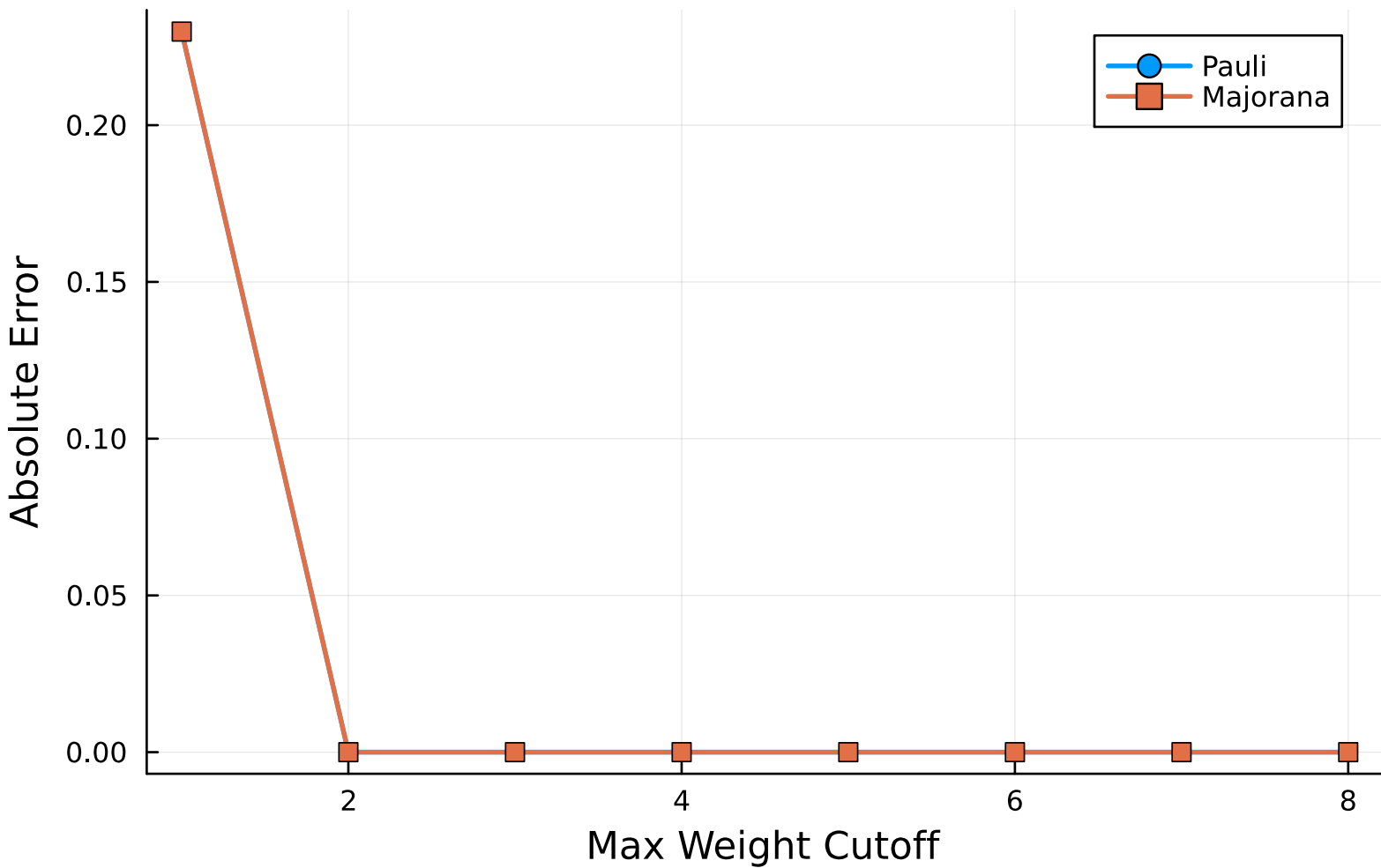
Error vs Max Weight (N=4, U=0)
