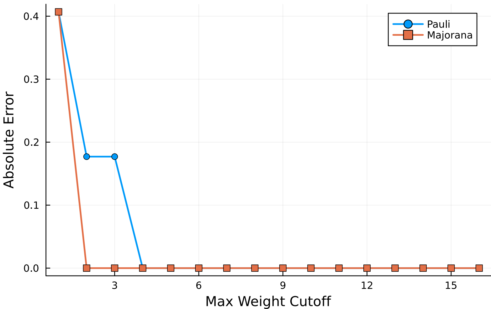
Error vs Max Weight (N=8, U=8)
